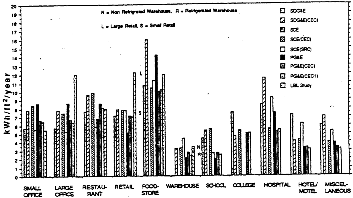
FIGURE 1 - LIGHTING EUIs COMPARISON
