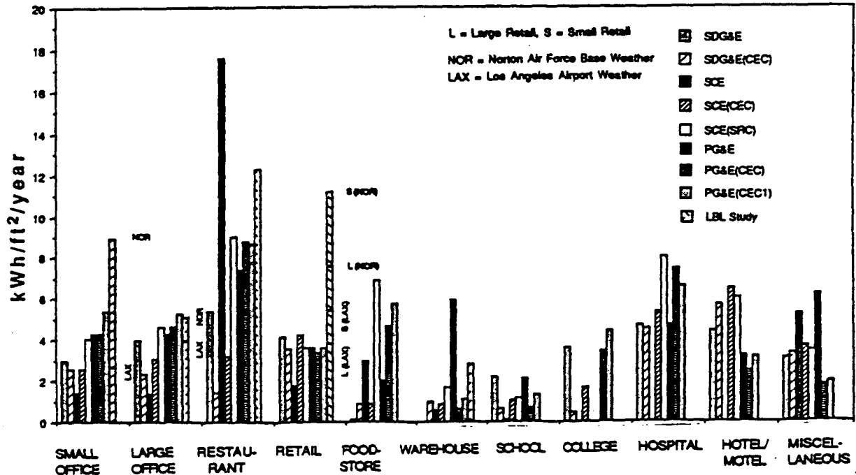
FIGURE 4 - COOLING EUIs COMPARISON
