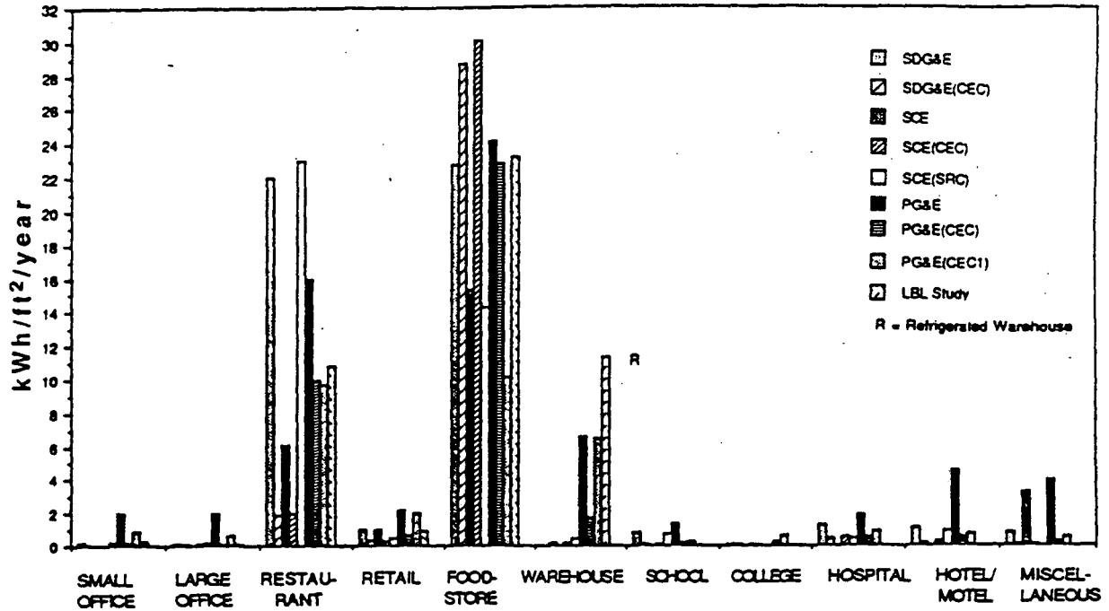
FIGURE 3 - REFRIGERATION EUIs COMPARISON
