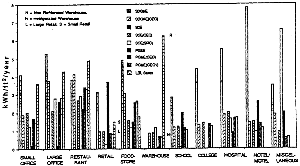
FIGURE 2 - ELECTRICAL MISCELLANEOUS EUIs COMPARISON
