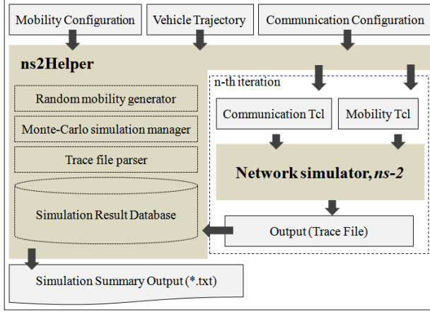
Figure 1. Simulation Framework
