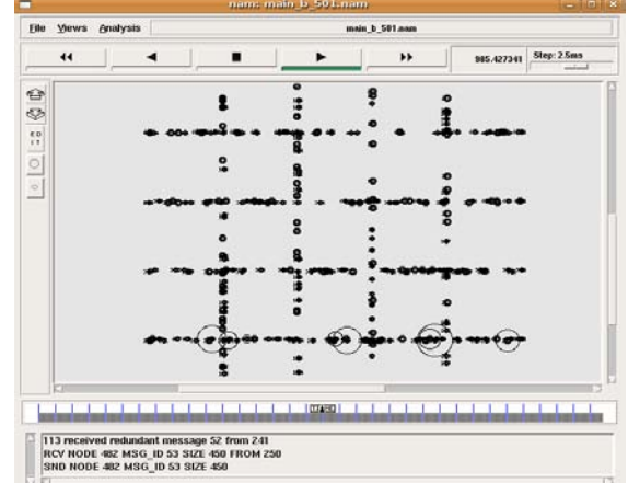
Figure 2. ns-2 simulation
