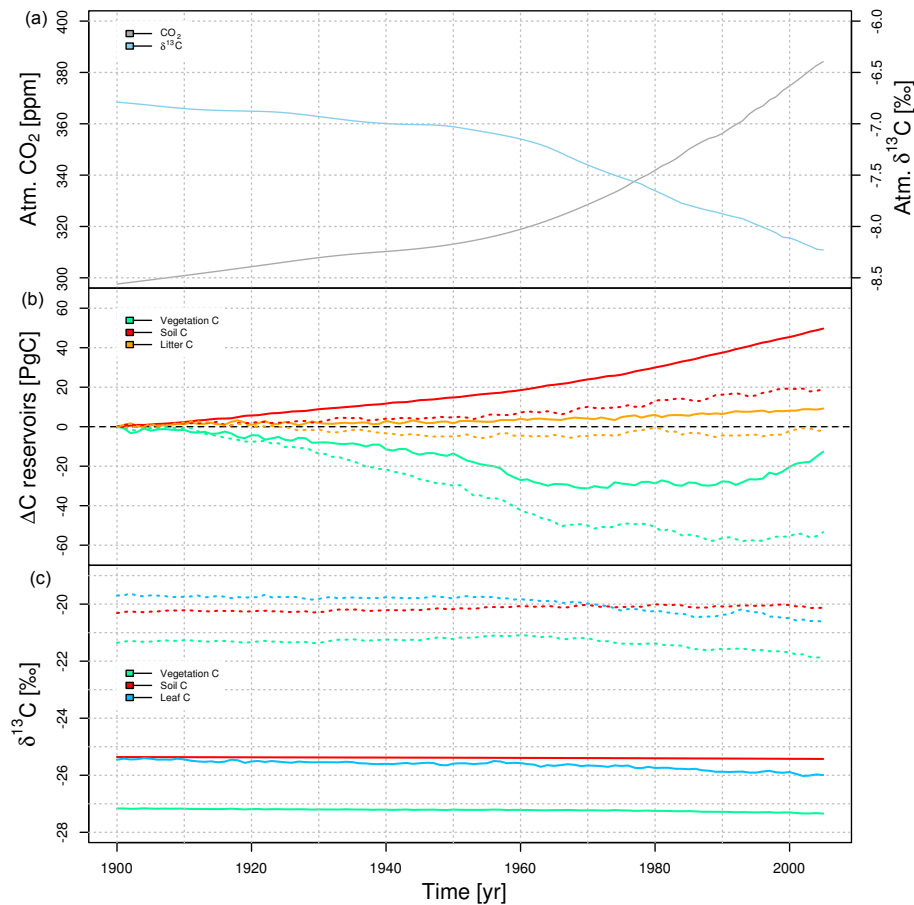
Figure 1. (a) Prescribed evolution of atmospheric CO 2 and its δ 13 C signature, (b) simulated changes in the global inventory of carbon stored in vegetation (green), litter (orange), soils (red), (c) Evolution of the global average (mass-weighted) δ 13 C signature of carbon in leaves, vegetation, and soils (CLM4.5: solid, LPX: dotted).
