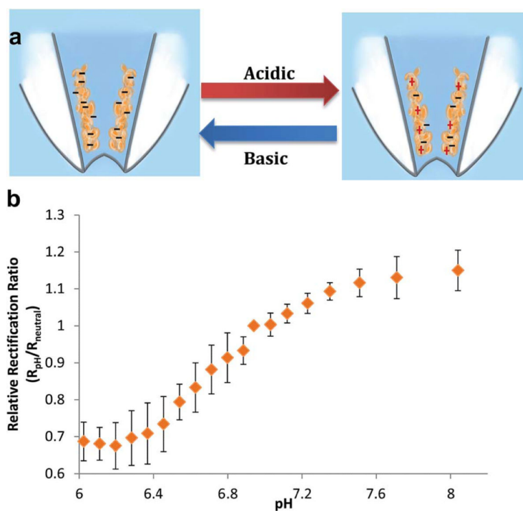
Fig. 2. (A) Schematic of the reversible changes in surface charge as a result of pH. (B) Calibration of chitosan-modified nanopipettes within the physiologically relevant pH range from 6.02 to 8.04. All data points are represented as relative rectification ratios at \pm 0.5 V vs. Ag/AgCl reference electrode. The error bars represent standard deviations for n = 4 replicate measurement. 0.1 M PBS was used as supporting electrolyte.
