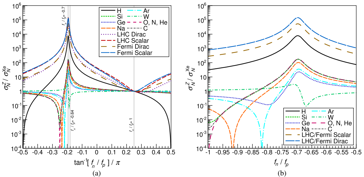
FIG. 4 (color online). Ratio of \sigma_N^Z in various experiments to \sigma_N^{Xe} . Results are shown as a function of f_n/f_p for scattering off various elements, as well as for LHC and Fermi determinations. In the xenophobic region the behavior of LHC and Fermi bounds for a given operator are visually identical. (a) Entire f_n/f_p range. (b) Xenophobic region.
