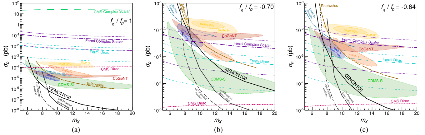
FIG. 1 (color online). Regions of interest and exclusion contours in the (m_X, \sigma_p) for neutron-to-proton coupling ratios f_n/f_p = 1 (left), f_n/f_p = -0.70 (center) and f_n/f_p = -0.64 (right). Plotted are the 90% CL ROIs for CDMS-Si [4], CoGeNT [2], and CDMS-Ge (Collar/Fields) [20], the 90% and 3\sigma ROIs for DAMA [1] as determined in Refs. [45,46], and exclusion contours from XENON100 [5,6], Edulweiss [47], and CDMS [17], and projected exclusion bounds from LUX [21]. Recent TEXONO [48] and CDEX-1 [49] bounds (not shown) are similar but moderately weaker than CDMS bounds over the mass interval shown. Also plotted are 90% CL exclusion contours from CMS and from the Fermi-LAT, assuming dark matter is either a complex scalar or Dirac fermion coupling only to first generation quarks through an effective contact interaction permitting unsuppressed spin-independent scattering and S -wave annihilation. The thin dot-dashed violet and dashed teal lines correspond to the systematic uncertainty in the Fermi-LAT bounds from astrophysical uncertainties for complex scalar and Dirac fermion candidates, respectively. In the center and right panels the CMS complex scalar exclusion bounds exceed the plotted range by between 1 and 2 orders of magnitude, and thus place no constraints on the disputed region.
