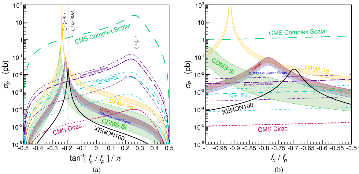
FIG. 3 (color online). Proton cross section for various experiments as a function of f_n/f_p for m_\chi = 8 GeV. Plotted are slices of the 90% CL ROIs for CDMS-Si [4], CoGeNT [19], and CDMS-Ge (Collar/Fields) [20], the 3\sigma ROI for DAMA [1], and exclusion contours for XENON100 [6]. Also plotted are 90% CL exclusion contours for CMS [39] and for the Fermi-LAT [31], assuming dark matter is either a complex scalar or Dirac fermion coupling only to first generation quarks through an effective contact interaction permitting unsuppressed spin-independent scattering and S -wave annihilation. The thin dot-dashed violet and dashed teal lines correspond to the systematic uncertainty in the Fermi-LAT bounds from astrophysical uncertainties for complex scalar and Dirac fermion candidates, respectively. (a) Entire f_n/f_p range. (b) Xenophobic region.
