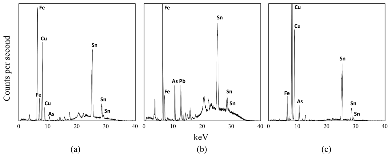
Figure 3.9: X-ray fluorescence analysis of crucible residues demonstrates melting and/or recycling practices. (a) Bo 2005: 293/305.263, (b) ETD 99/110, (c) ETD 96/218. Adapted from Lehner and Schachner (in press: fig. 10)
