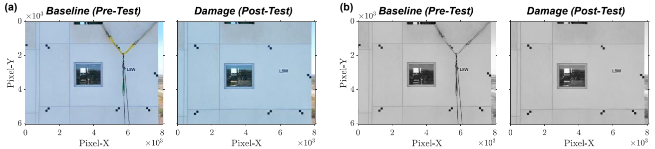
Fig. 3 (a) Raw RGB images captured by UAV, and (b) Converted grayscale images.
