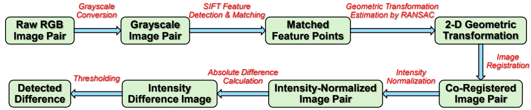
Fig. 2 Flowchart of the proposed damage detection methodology.
