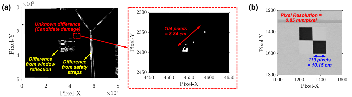
Fig. 6 (a) Detected difference with zoom-in view for candidate damage, and (b) Pixel resolution calculation using features with known dimensions from the pre-test grayscale image.
