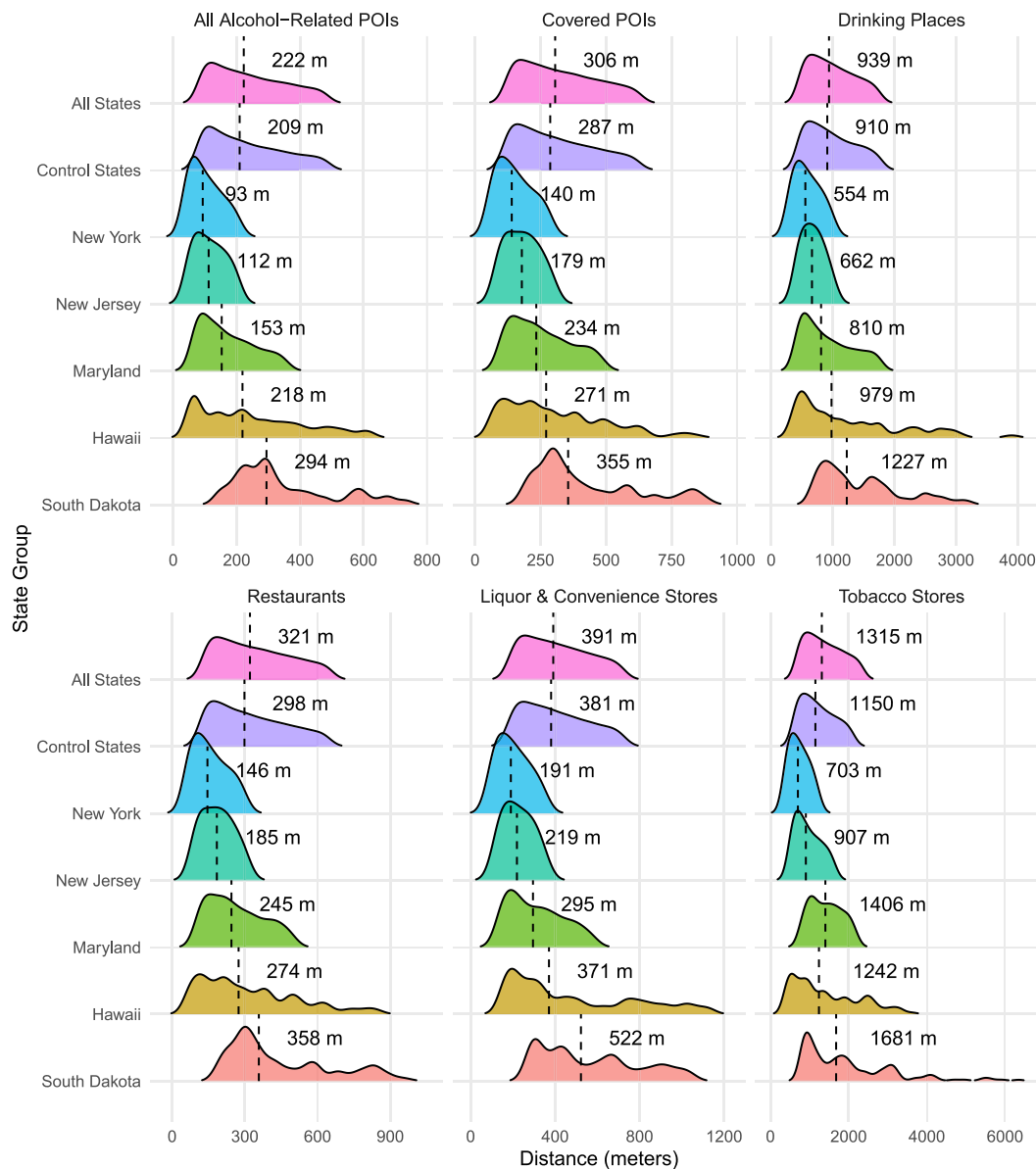
Fig. 2. Distributions of median distances between shootings and POIs, by subcategory, across states.
