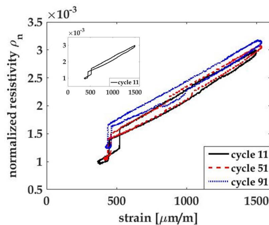
Figure 6. The hysteresis plot of the MWCNT-Pluronic-PVDF thin film was acquired from the 100-cycle test.
