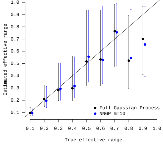
(b) \sigma^2 = 0.1
