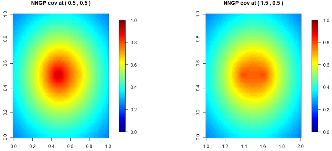
Figure A8: NNGP covariance function using a grid \mathcal{S}
