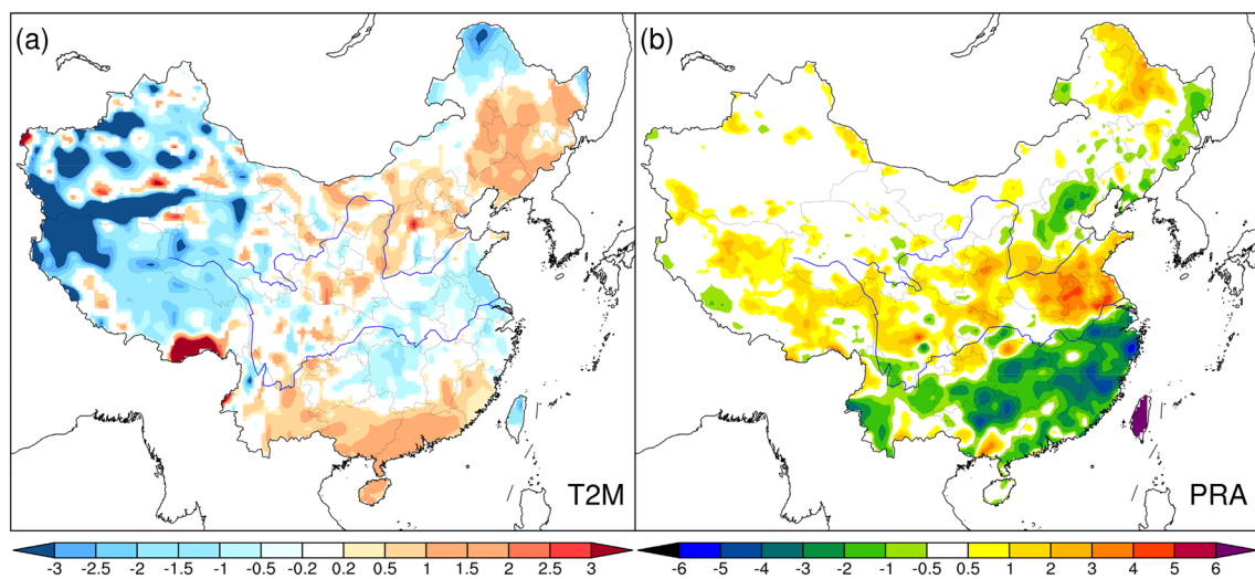
Fig. 2 Observed a May temperature (°C) and b summer precipitation (mm day -1 ) anomalies in 2003
