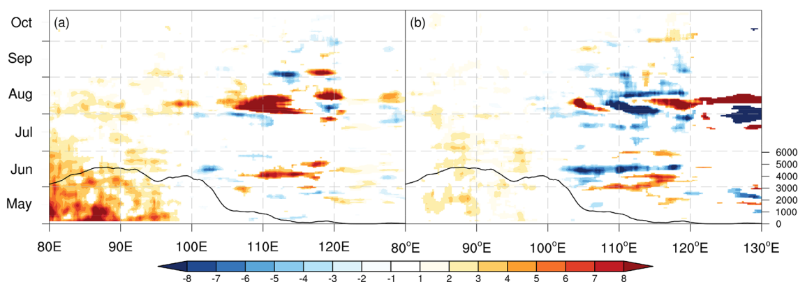
Fig. 8 CWRW simulated time-longitude variations of 27° N–37° N latitudinal mean surface a sensible and b latent heat flux ( \text{W m}^{-2} ) differences between the warm start IbTpWc and IbTnWn. The black lines depict the latitudinal mean terrain elevation (m), using the scale on the right
