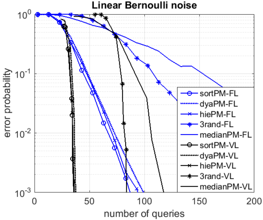
Figure 2.3: Error probability vs. number of queries: linear noise case We set resolution \frac{1}{\delta} = 2^{15} and Bernoulli noise with linear flipping probability p[\delta|S|] = 0.1 + \delta|S|/2
