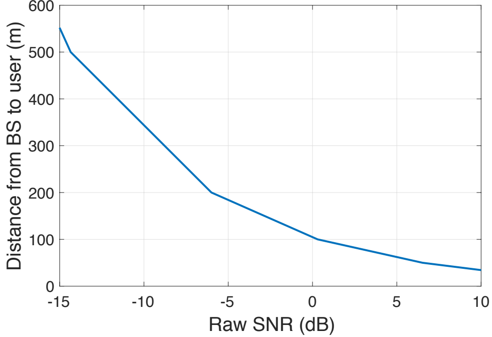
Figure 4.6: Relationship between raw SNR P/\sigma^2 and distance from BS to user. This relationship is generated by the 3GPP TR 38.901 UMi LOS pathloss channel model (summarized in [36]), with 73GHz carrier frequency, 23 dBm maximum user power, -174 dBm/Hz thermal noise density, 5 dB receiver noise figure at BS, and a bandwidth of 100 MHz.
