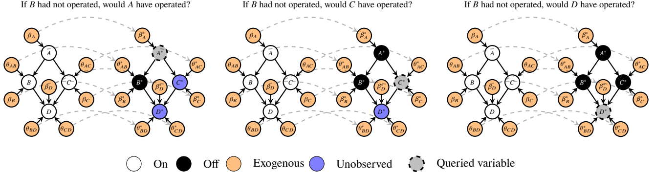
Figure 3: Example of sequential commitment to previous judgments in a sequence of counterfactual queries (from left to right) in the firing-squad scenario. Each query specifies counterfactual observations in the twin model including the actual world observations ( A = B = C = D = 1 ), the counterfactual constraint ( B^* = 0 ), and previous judgments – if any – at query time. Commitment means adding the previous judgments to the counterfactual observation set for the current query. In this example, the participant answers ‘No’ to the first two queries in the (ACD) order. The ‘No’ to the first query about A^* is carried over to the second query, and the ‘No’ to the query about C^* is carried over to the third query, making it likely that the answer to that query will be ‘No’ as well.
