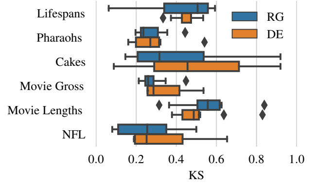
Figure 4: KS distance between environmental distributions and elicitation data.
