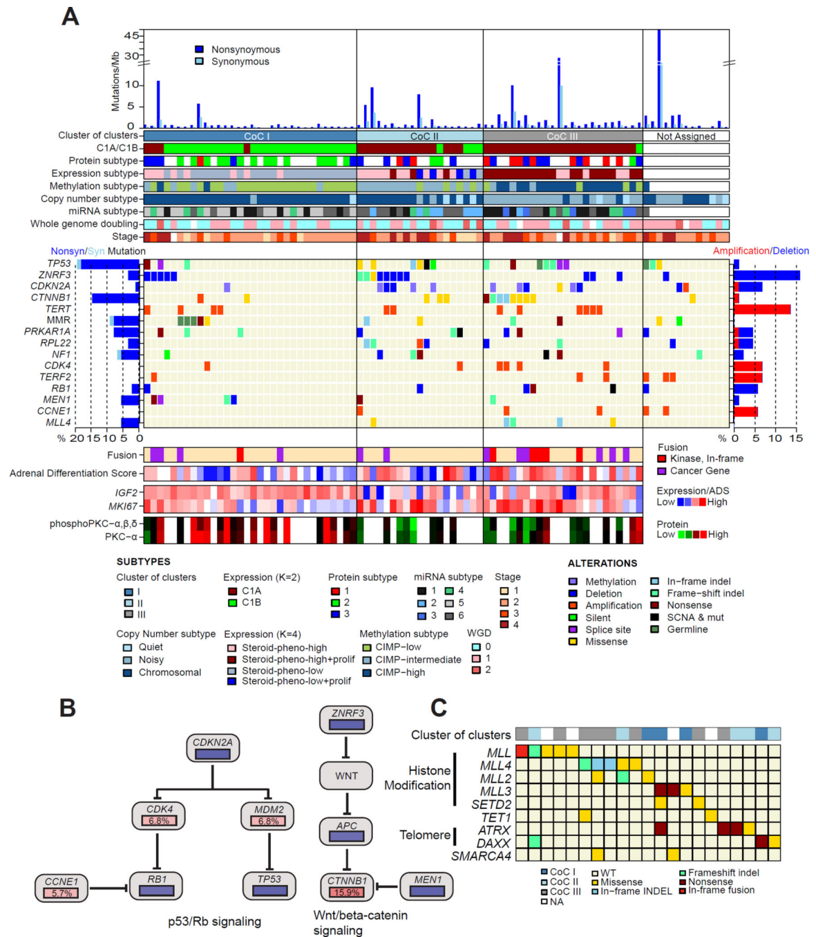
Figure 5. Genomic landscape of ACC
