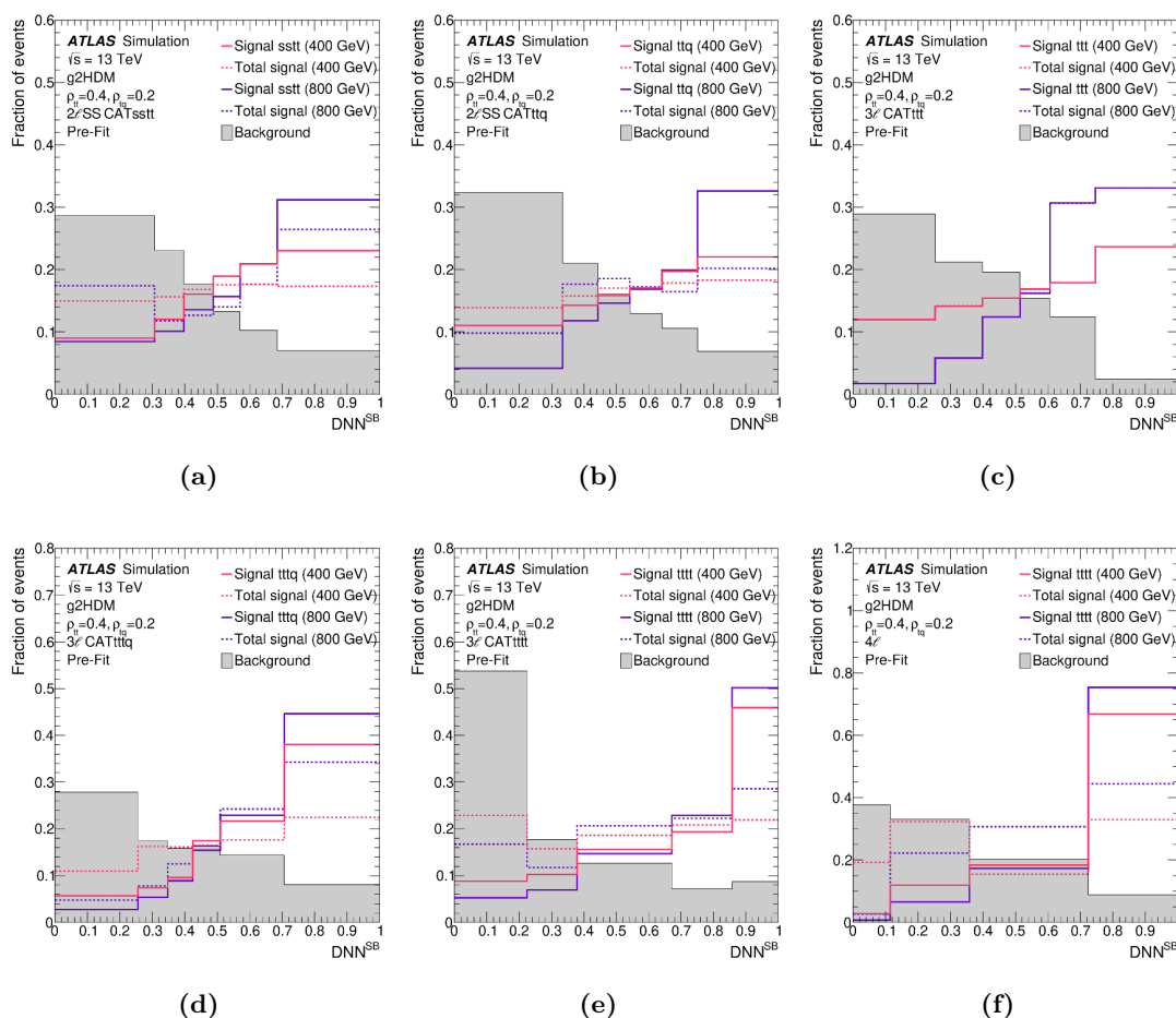
Figure 5. Comparison of the DNN^{SB} distribution of the targeted signal (solid line), the total signal (dashed line) and the background (filled grey area) in the (a) 2 \ell SS CAT ss \bar{t}t , (b) 2 \ell SS CAT ttq, (c) 3 \ell CAT ttt, (d) 3 \ell CAT tttq, (e) 3 \ell CAT tttt, and (f) 4 \ell categories, for an assumed m_H = 400 GeV (pink) and m_H = 800 GeV (violet), with couplings \rho_{tt} = 0.4 and \rho_{tq} = 0.2 . All distributions are normalised to unity.
