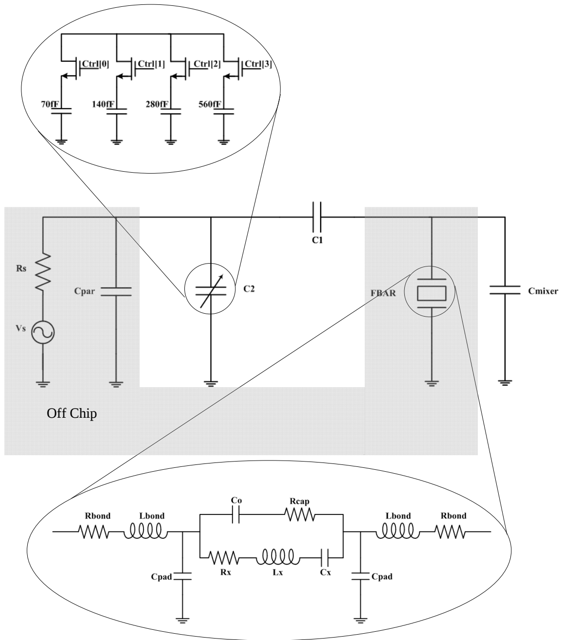
Figure 3.20 Complete schematic of FBAR resonator input matching network with parasitics
