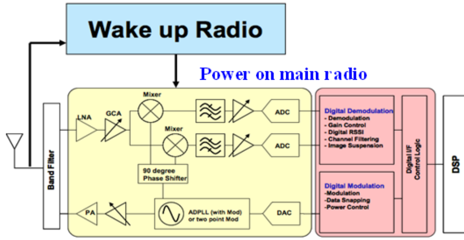
Figure 2.1 System Integration with WuRx
