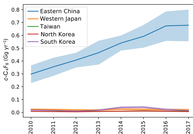
Figure 6. c -C 4 F 8 emissions in eastern Asia as determined by the NAME-HB regional inversion of measurements at the Gosan station, Jeju Island, South Korea, are dominated by emissions from China (blue). Emissions from western Japan (orange) and South Korea (violet) are much smaller; the latter show a small maximum in 2014 and 2015. Emissions from Taiwan (green) and North Korea (red) are also small. Shadings represent uncertainty bands of emissions.
