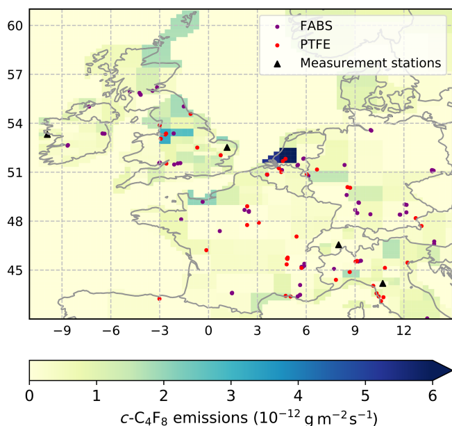
Figure 8. Mean c -C 4 F 8 emission strength (shades of green and blue, 10^{-12} \text{ g m}^{-2} \text{ s}^{-1} ) in northwestern Europe (42 to 59° N and -11 to 15° E) from 2013 to 2017 determined by the IN-TEM inversion from measurements at four sites (Mace Head, Ireland, Tacolneston, United Kingdom, Jungfrauoch, Switzerland, and Monte Cimone, Italy, black triangles). Also shown are potential industrial emitters of c -C 4 F 8 . Locations of potential TFE/HFP/PTFE/FEP production facilities (red dots) are based on company websites (3M, Chemours, Daikin, DuPont, Saint-Gobain, and Solvay) and are much less certain than the corresponding location information for eastern Asia. Also shown are semiconductor fabrication plants (purple dots, https://en.wikipedia.org/wiki/List_of_semiconductor_fabrication_plants , last access: 3 December 2018; http://www.10stripe.com/featured/map/semiconductor-fabs.php , last access: 3 December 2018; and other sources).
