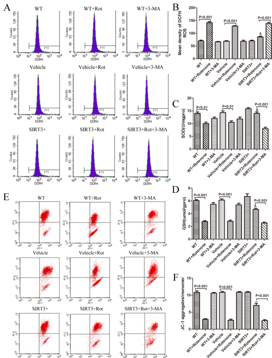
Figure 5. SIRT3 upregulates intracellular SOD and GSH levels, prevents rotenone-induced ROS generation and MMP collapse in SH-SY5Y cells by upregulating autophagy. The SH-SY5Y cells with or without SIRT3 overexpression cultured in serum-free growth medium were treated with 60 \mu M rotenone for 24 h. Five millimolar 3-MA was added 1h before rotenone. The cells were harvested and stained with DCFH-DA. (A) ROS levels were measured by a fluorescence-activated cell sorter. (B) Bar graph shows the quantification of ROS levels. Mean \pm SEM, n=3. \delta : P < 0.001 vs. Vehicle+Rotenone. The cells were collected for quantification of intracellular SOD (C), GSH (D) using the corresponding detecting kits. Mean \pm SEM, n=3. #: P < 0.05 vs. Vehicle+Rotenone. \delta : P < 0.001 vs. Vehicle+Rotenone. (E) MMP was measured by JC-1 aggregates/monomer using a flow cytometer. (F) The bar graph shows the quantification of JC-1 aggregates/monomer levels in each group. Mean \pm SEM, n=3. \sigma : P < 0.001 vs. Vehicle+Rotenone.
