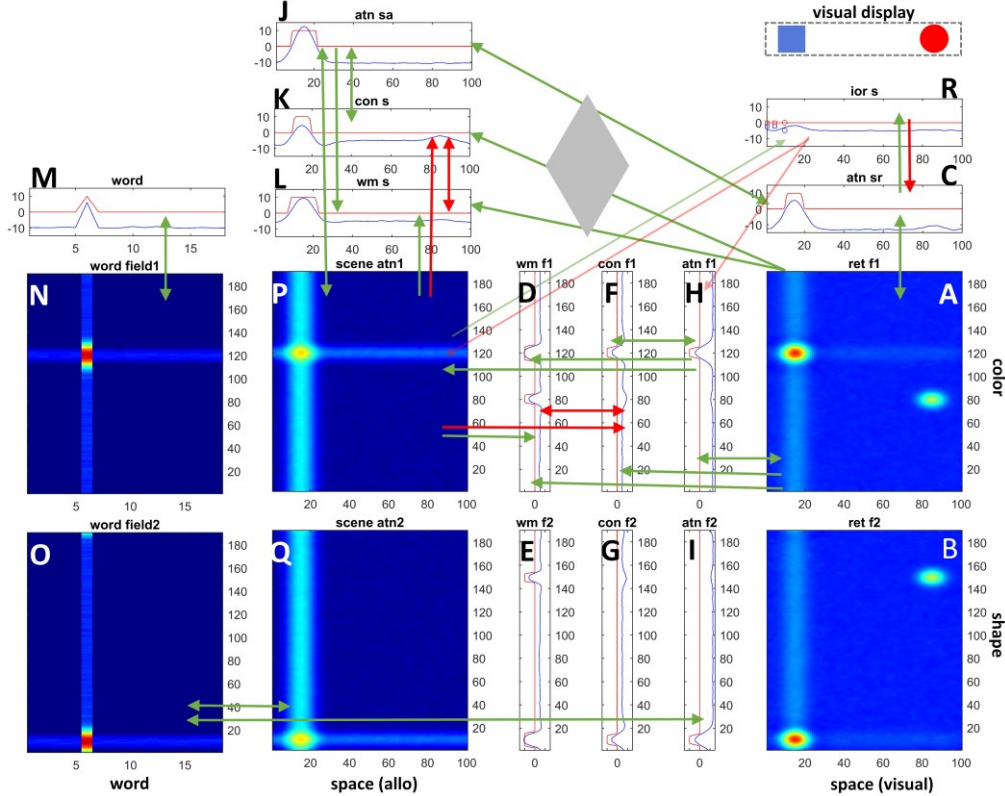
Figure 1: WOLVES model architecture. Rectangles A-R represent component DNFs and arrows represent uni- /bi-directional (green: excitatory, red: inhibitory) connectivity in the model. See text for figure description.
