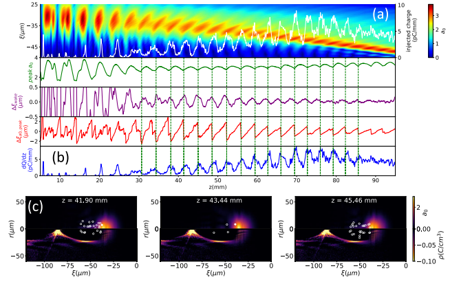
FIG. 6. FBPIC simulation with particle tracking, for the same parameters as the blue curve of Fig. 1(a). (a) On-axis evolution of the laser envelope ( a_0 ) in the light frame (computation window, \xi = z - v_g t ), showing the periodic motion of the laser pulse peak and pulse retreat in the light frame. The white curve is a histogram of electron injection locations contributing to the bunch at z = 10 cm with electrons >50 MeV. (b) Lineouts of pulse and wake parameters vs propagation distance (see text). Green curve: peak a_0 in moving window. Purple curve: relative position of the back of the wake, \Delta\xi_{\text{wake}} = \xi_{\text{wake}} - \langle \xi_{\text{wake}} \rangle_{1 \text{ cm}} . Red curve: relative position of peak a_0 , \Delta\xi_{a_0, \text{peak}} = \xi_{a_0, \text{peak}} - \langle \xi_{a_0, \text{peak}} \rangle_{1 \text{ cm}} . Blue curve: replot of white curve from panel (a). (c) Laser field envelope (top half of frame) and plasma density (bottom half) overlaid with injected electron initial locations (white dots and circles) over a full cycle of beating, showing two injection maxima and a minimum. The dots mark likely birth locations of trapped electrons in a given frame.
