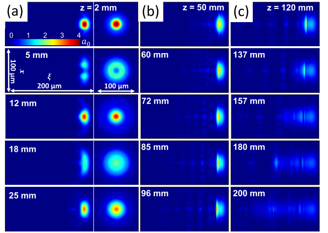
FIG. 2. Evolution of LWFA drive pulse corresponding to the blue curve in Fig. 1(a). Column (a) for stage I, plots x\xi slices of the field magnitude a_0 on the left and the \xi -integrated mode on the right, where \xi = z - ct is the space coordinate in the moving computation frame. Longitudinal positions denoted on the frames are marked by the blue crosses in Fig. 1(a). Column (b), for stage II, plots x\xi slices of a_0 for the longitudinal positions marked by the blue stars. Column (c), for stage III, plots x\xi slices of a_0 for the longitudinal positions marked by the open circles in Fig. 1(a). All slices and profiles are normalized to the maximum at z = 2 \text{ mm} .
