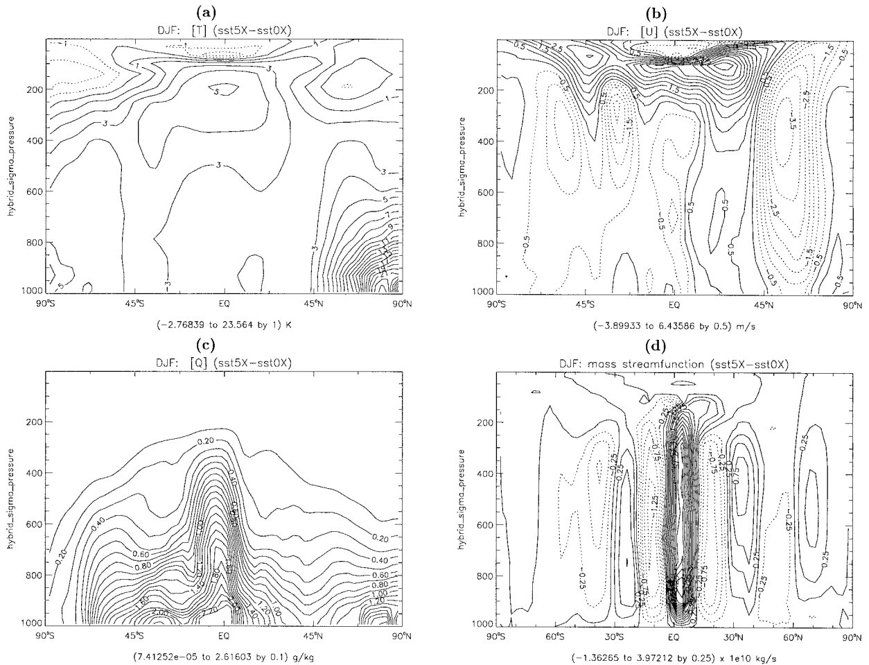
FIG. 4. DJF-mean, zonally averaged response (deviations from 0X) for the 5X case. Negative contours are dashed. (a) Temperature response. Contour interval is 1 K. (b) Zonal wind response in meters per second. Contour interval is 0.5. (c) Specific humidity response in grams per kilogram. Contour interval is 0.1. (d) Mass streamfunction in 10^{10} kilograms per second. Contour interval is 0.25.
