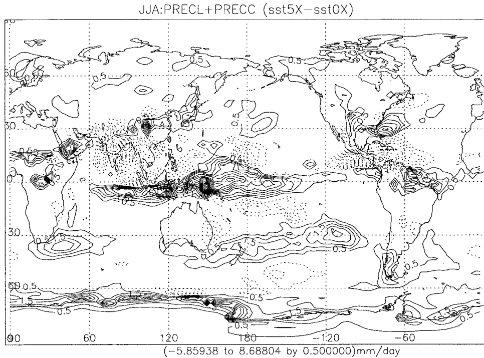
FIG. 13. JJA-mean response in rainfall for 5X ( \text{mm day}^{-1} ). Negative contours are dashed. Contour interval is 0.5. Zero contour has been omitted.
