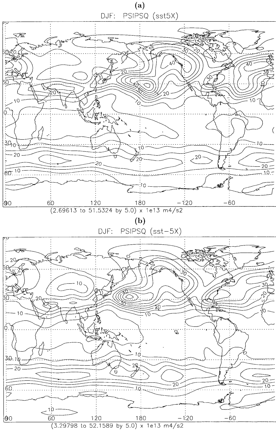
FIG. 8. DJF-mean high-frequency filtered transient eddy streamfunction variance ( 10^{13} \text{ m}^4 \text{ s}^{-2} ). Contour interval is 5. (a) 5X. (b) -5X.
