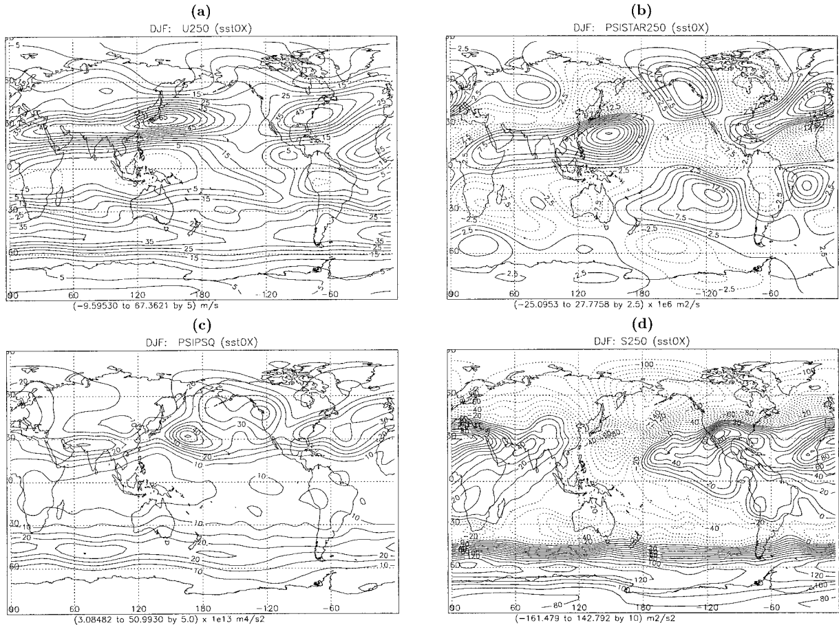
FIG. 2. DJF-mean fields for the control case (0X) on the 250-hPa surface. Negative contours are dashed. (a) Zonal wind ( \text{m s}^{-1} ), contour interval is 5. (b) Eddy streamfunction ( \overline{\psi'^2} , 10^6 \text{ m}^2 \text{ s}^{-1} ), contour interval is 2.5. (c) High-frequency filtered transient eddy streamfunction variance ( 10^{13} \text{ m}^4 \text{ s}^{-2} ), contour interval is 5. (d) Barotropic forcing of the mean streamfunction by the high-frequency filtered transient eddies ( \text{m}^2 \text{ s}^{-2} ), contour interval is 10.
