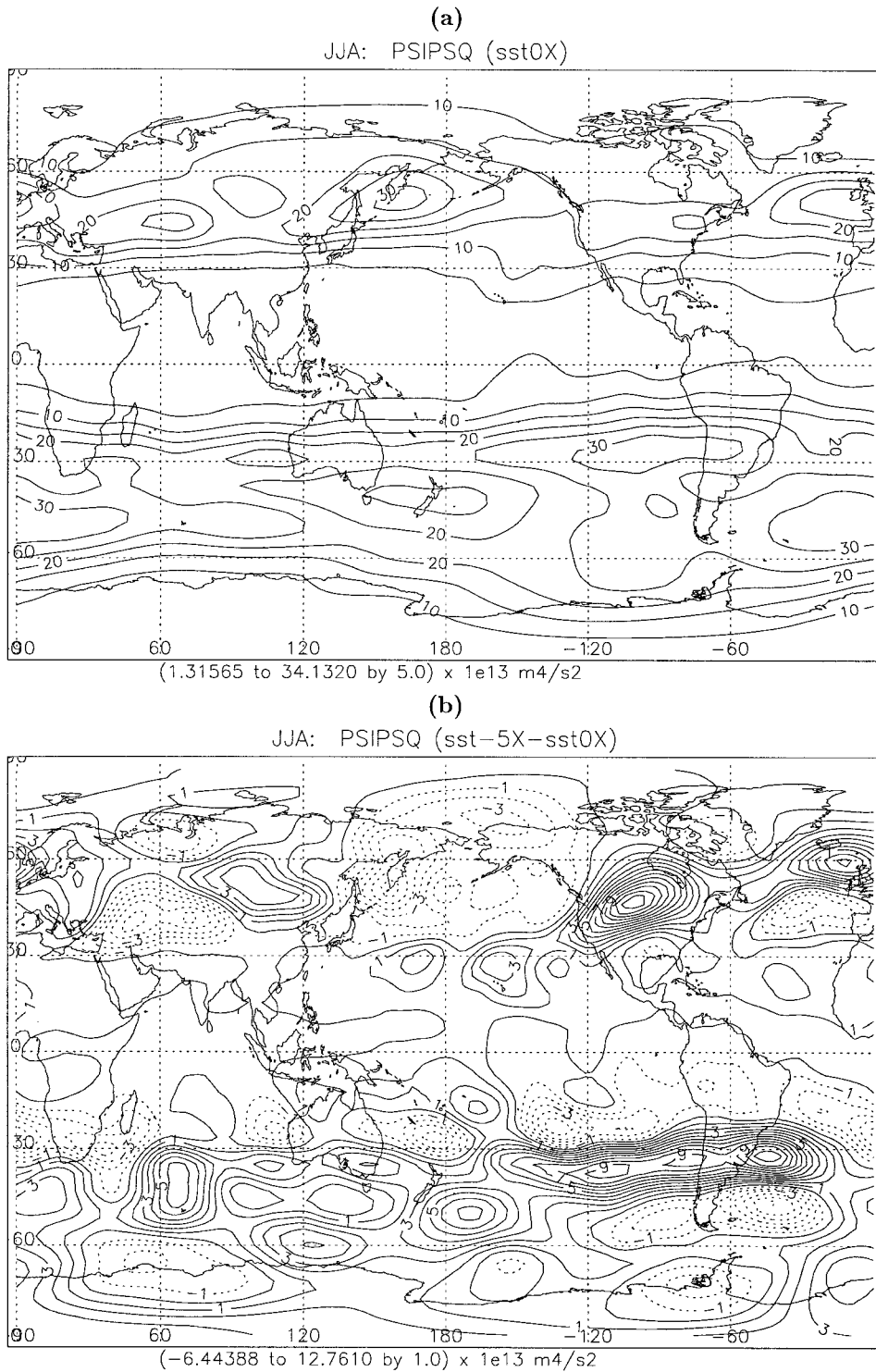
FIG. 15. JJA-mean fields on the 250-hPa surface. (a) 0X transient eddy streamfunction variance ( 10^{13} \text{ m}^4 \text{ s}^{-2} ). Contour interval is 5. (b) -5X response of transient eddy streamfunction variance ( 10^{13} \text{ m}^4 \text{ s}^{-2} ). Negative contours are dashed. Contour interval is 1.
