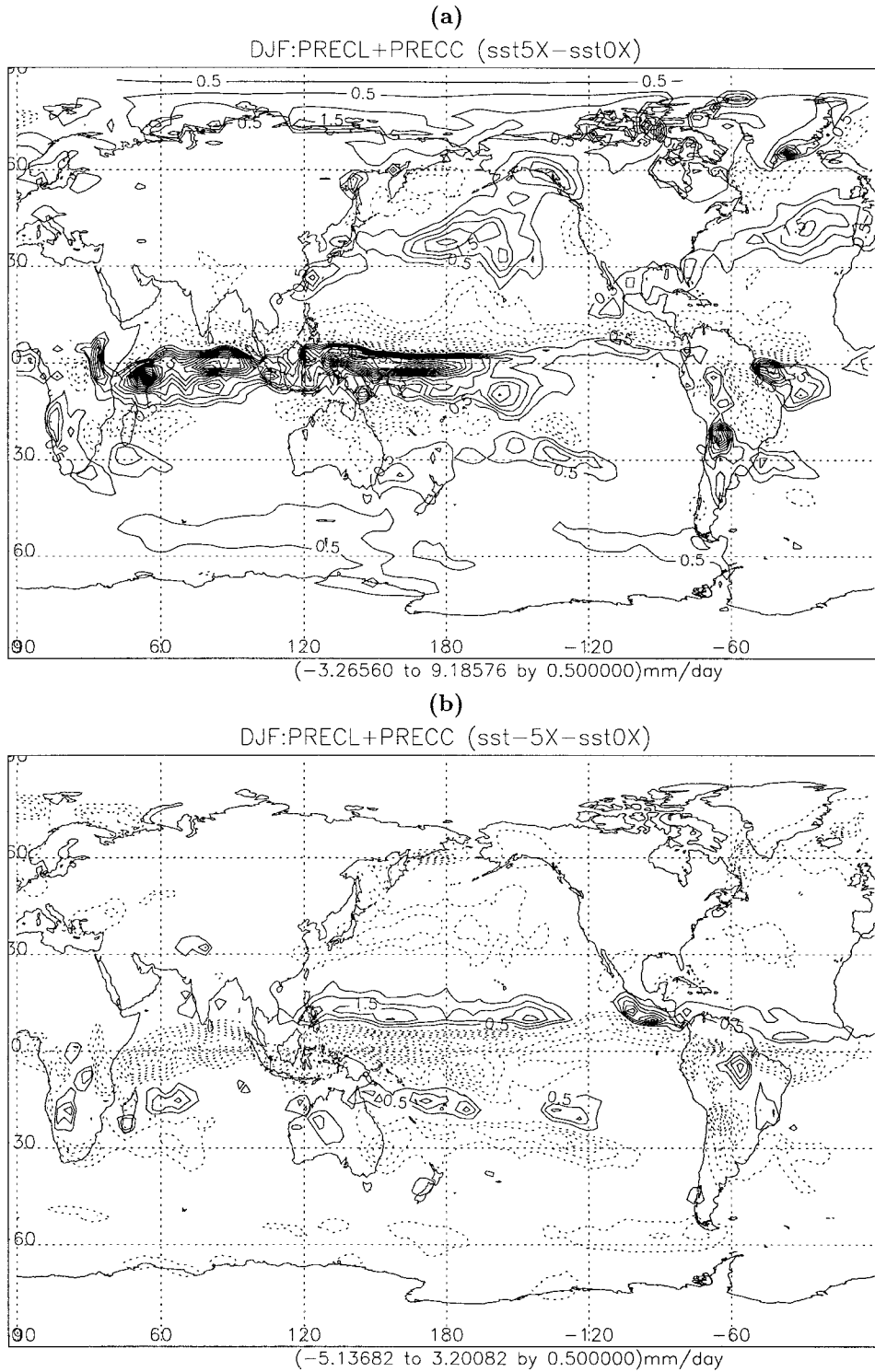
FIG. 5. DJF-mean response in rainfall ( \text{mm day}^{-1} ). Negative contours are dashed. Contour interval is 0.5. The zero contour has been omitted. (a) 5X-0X. (b) -5X-0X.
