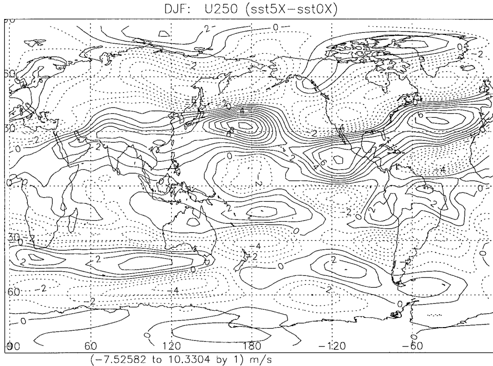
FIG. 6. DJF-mean response for 5X in 250-hPa zonal wind ( \text{m s}^{-1} ). Negative contours are dashed. Contour interval is 1.
