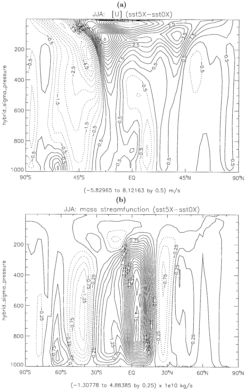
FIG. 12. JJA-mean, zonally averaged response for 5X (deviations from 0X). Negative contours are dashed. (a) Zonal wind ( \text{m s}^{-1} ), contour interval is 0.5. (b) Mass streamfunction [ (10^{10} \text{ kg s}^{-1}) , contour interval is 0.25].
