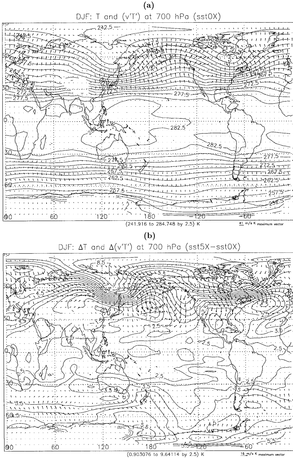
FIG. 10. DJF-mean fields on the 700-hPa surface, smoothed to T21 horizontal resolution. (a) 0X temperature (contour interval is 2.5 K) and high-frequency filtered transient temperature flux [vectors (m K s -1 )]. Vector, shown in lower-right-hand corner, has the value 41. (b) The 5X temperature response [contours (K), contour interval is 0.5], and response of high-frequency filtered transient temperature flux [(vectors (m K s -1 )), vector has value 16.
