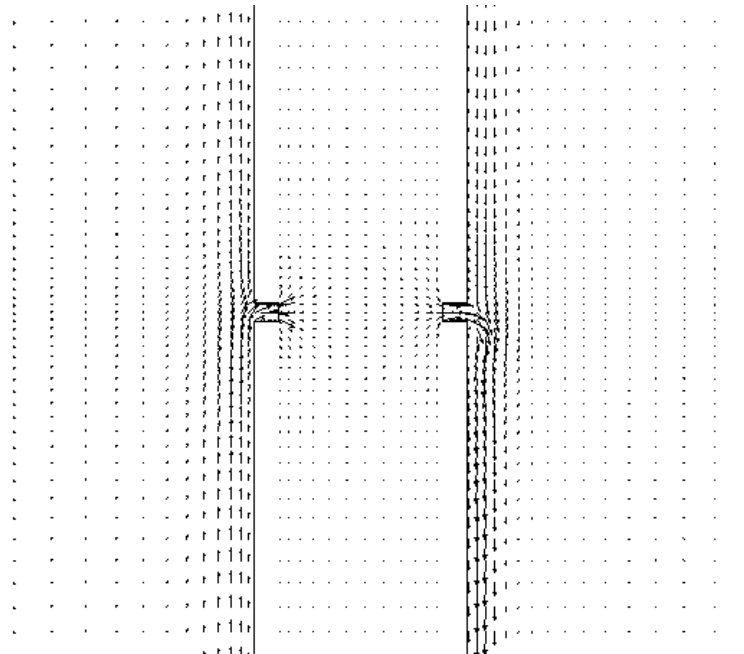
Figure 6. Air flow velocity vectors from a two-dimensional CFD simulation of the wall with a straight through leakage path (wall 2). Note that this figure concentrates on the areas around the leaks and represents only a fraction of the total wall height.
