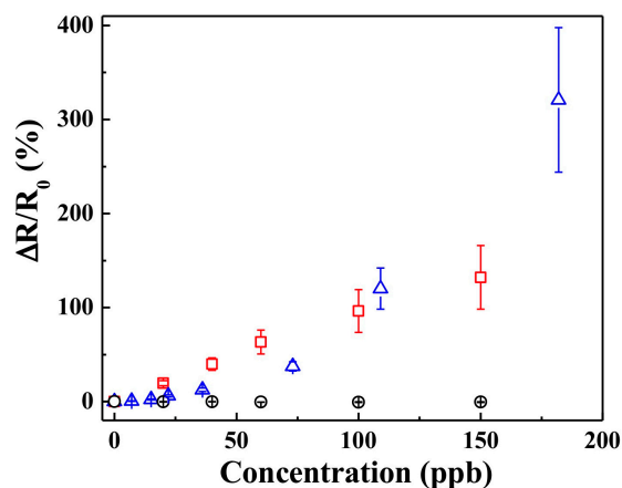
Figure 1. Normalized responses from the pristine polyaniline (PANI) sensors: (red/ \square ) NO 2 , (blue/ \Delta ) O 3 , and (black/ \circ ) SO 2 ; 25 °C; 50% relative humidity (RH). Data points are average of responses from three independent sensors, and error bars represent \pm 1 standard deviation.
