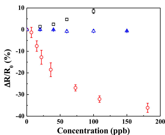
Figure 4. Selectivity of KI-PANI sensor towards \text{O}_3 (red/○) with respect to other interfering analytes \text{NO}_2 (black/□) and \text{SO}_2 (blue/△) in terms of sensing response ( \Delta R/R_0 ) at various analyte concentrations. Data points are average of responses from three independent sensors, and error bars represent \pm 1 standard deviation.
