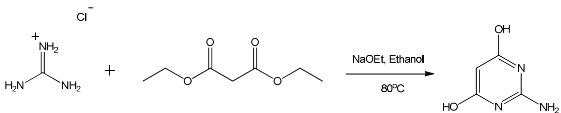
Scheme 4.21 25 : Synthesis of 6-hydroxyisocytosine.
