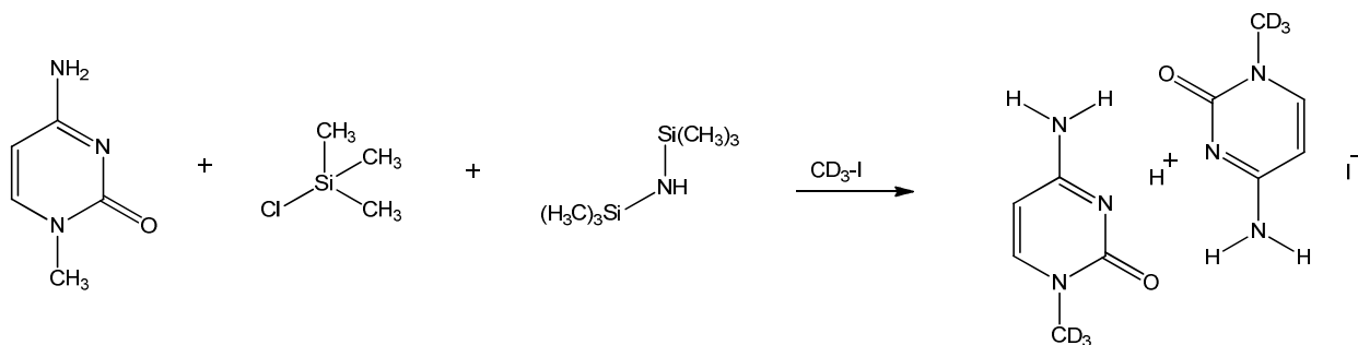
Scheme 2.10: Synthesis of the 1-methylcytosine- d 6 PBD iodide salt.
