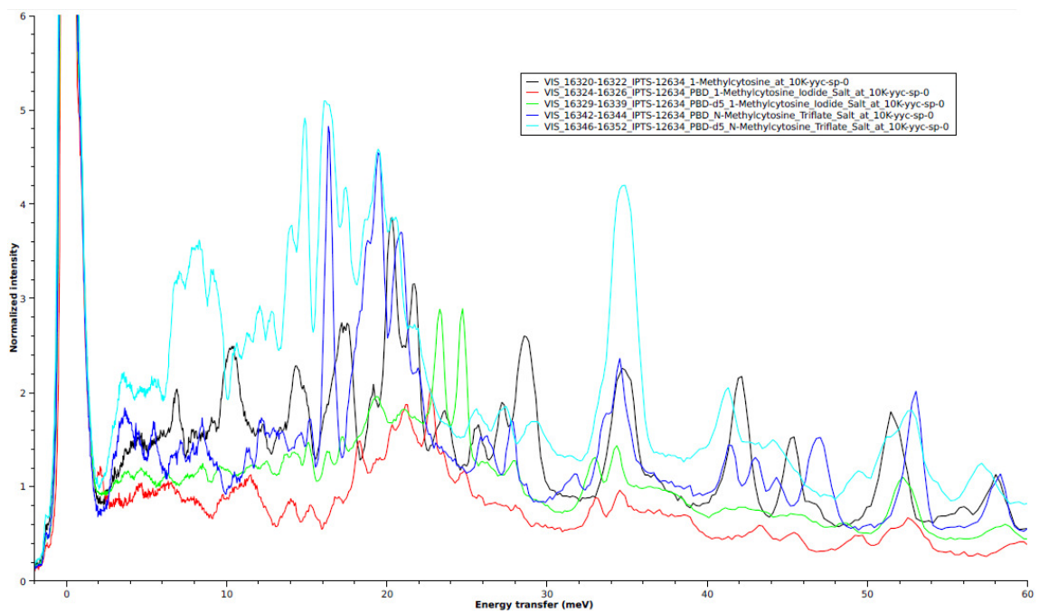
Figure 2.43: Neutron scattering spectra of 1-methylcytosine (black trace), 1-Iodide (red trace), 1-Iodide-d 5 (green trace), 1-Triflate (dark blue trace), and 1-Triflate-d 5 (light blue trace) recorded at SNS by Dr. Luke Daemen.
