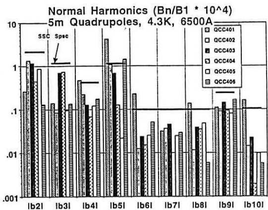
Figure 11b: Normalized Normal Multipole Components (E-4 units for Several Magnets)
