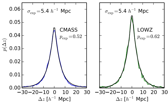
Figure 10. The probability distribution of apparent line-of-sight separations for pairs of galaxies in the same fibre collision group and for which both have good redshifts. The left panel uses pairs of CMASS targets and the right panel uses pairs of LOWZ targets. Both distributions can be fit with the sum of a background term and an exponential: ae^{-|\Delta z|/\sigma} + b in the range |\Delta z| < 50 \text{ h}^{-1} \text{ Mpc} . A total of 52% (62%) of the CMASS (LOWZ) pairs contribute to the exponential term. The best fit width \sigma of the exponential component is 5.4 \text{ h}^{-1} \text{ Mpc} for both CMASS and LOWZ targets.
