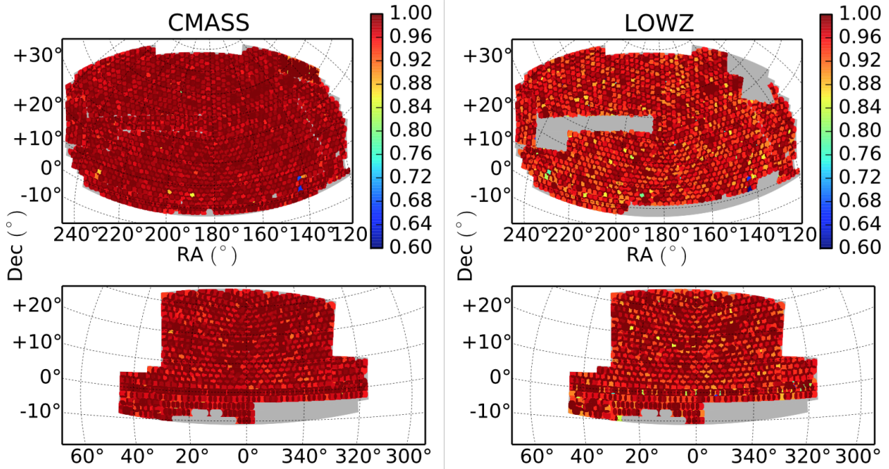
Figure 8. Completeness maps for both the LOWZ and CMASS samples in the north and south Galactic caps. The mean completeness is 98.8% for the CMASS sample shown in the left panels, and 97.2% for the LOWZ sample in the right-hand panels. Gaps correspond to early chunks as shown in Fig. A1. Each patch of different colour corresponds to a plate, with the colour determined by the completeness of that plate. This is surrounded by the higher completeness regions that overlap that plate with other plates. This leaves a pattern that looks like a darker, higher-completeness mesh, covering the survey.
