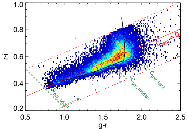
Figure 3. Density plot of LOWZ galaxies in the (g-r, r-i) colour plane; red corresponds to higher density and dark blue to lower density, in an arbitrary normalisation and linear scale. Redshift increases rightwards and upwards along the galaxies locus, starting at z \approx 0.1 on the bottom left corner. The knee on the galaxy locus is caused by the 4000 Å break transitioning between the g- and r- band filters, and happens at z \approx 0.4 . The colours c_{\perp} and c_{||} are simple rotations of this colour plane, and trace the position of a target in parallel and perpendicular, respectively, to the data locus. The black thick line represents the passively evolving LRG model of Maraston et al. (2009). The green and red dashed lines are the colour and magnitude targeting cuts – see the main text for details. The few targets seen outside of the selection cut are due to differences in the targeting and final photometry, see Section 2.
