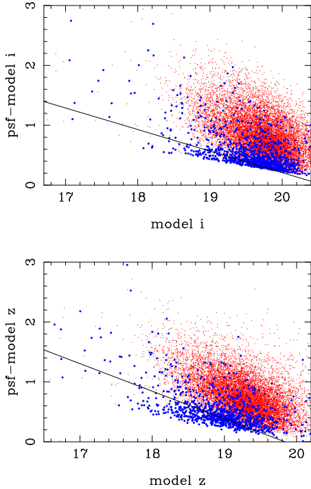
Figure 5. The distribution of spectroscopically confirmed stars (large blue points) and galaxies (small red points) in the psf\text{-model } i vs model\ i (top) and z\text{-band} (bottom) planes selected in the CMASS sample of the commissioning data. The black lines are the linear cuts that remove the most spectroscopically confirmed stars whilst removing less than 1% of the galaxies. The z\text{-band} cut was added to the original i\text{-band} cut targeting from chunk 3 onwards.
