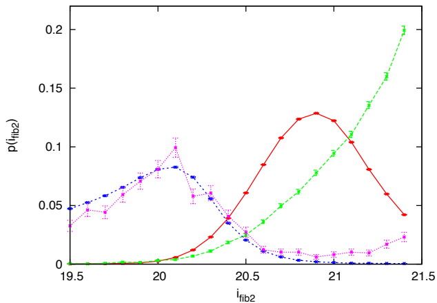
Figure 7. Normalised i_{\text{fib}2} distributions of redshift failures (green, dashed) and redshift successes (red, solid) for the CMASS sample. Redshift failures constitute 1.8% of the CMASS targets observed by SDSS-III BOSS. These are contrasted against normalised distributions for the LOWZ sample of redshift failures (pink, dotted) and redshift successes (blue, dashed). Error bars were calculated assuming Poisson statistics. Note that some LOWZ galaxies have i_{\text{fib}2} < 19.5 , which is why the normalisation for LOWZ curves looks lower than for CMASS.
