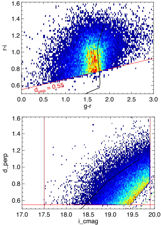
Figure 4. Both panels show density plots of CMASS galaxies; red corresponds to higher density and dark blue to lower density in an arbitrary normalisation and linear scale. The black thick line shows the passively evolving LRG model of Maraston et al. (2009). Top: redshift increases upwards, starting at z \simeq 0.4 at d_{\perp} = 0.55 . Bottom: the sliding cut in d_{\perp} with i -band magnitude, designed to select an approximately stellar-mass complete sample. Stellar mass increases with the perpendicular distance to the sliding cut, represented here by the red dashed line - see Maraston et al. (2013) for details. The green dashed line shows the sliding cut adopted for the CMASS SPARSE sample (see Section 3.4). Vertical solid lines show the magnitude limits. On both panels, the small fraction of targets that lie outside of the selection cut are due to differences in the targeting and final photometry, see Section 2. Only chunks greater than 6 are shown.
