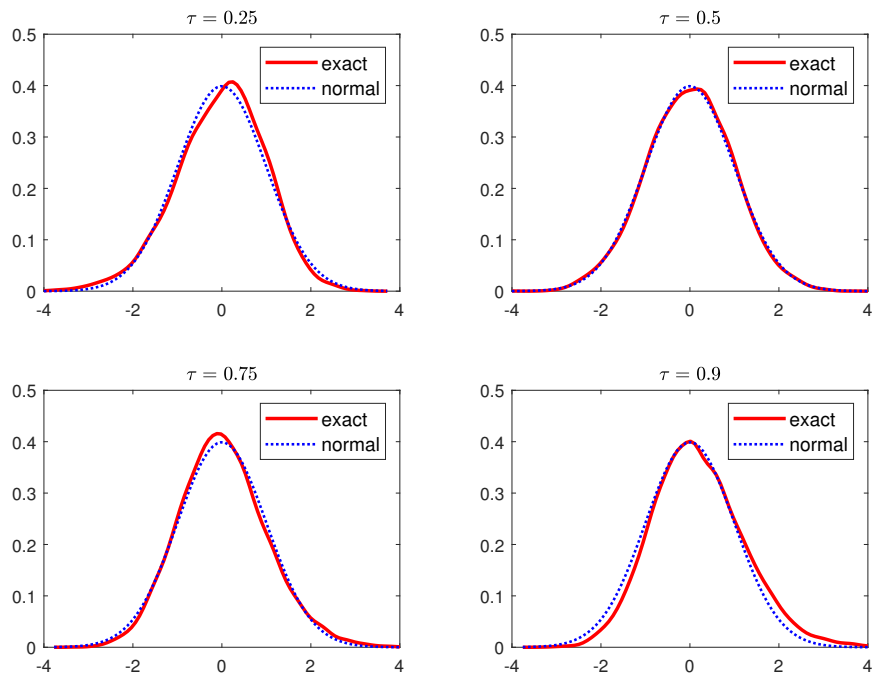
Figure 4: Finite sample exact distribution of the studentized scale effect statistic when \beta = 0.75 , \sigma_X^2 = 1 , and n = 1000 .
