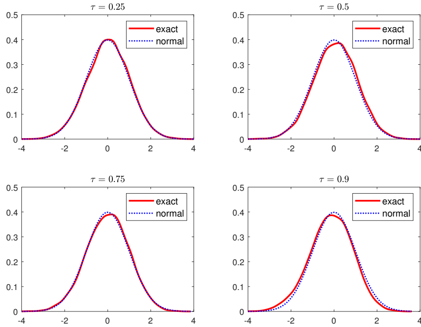
Figure 1: Finite sample exact distribution of the studentized location effect statistic when \beta = 0.25 , \sigma_X^2 = 1 , and n = 1000 .
