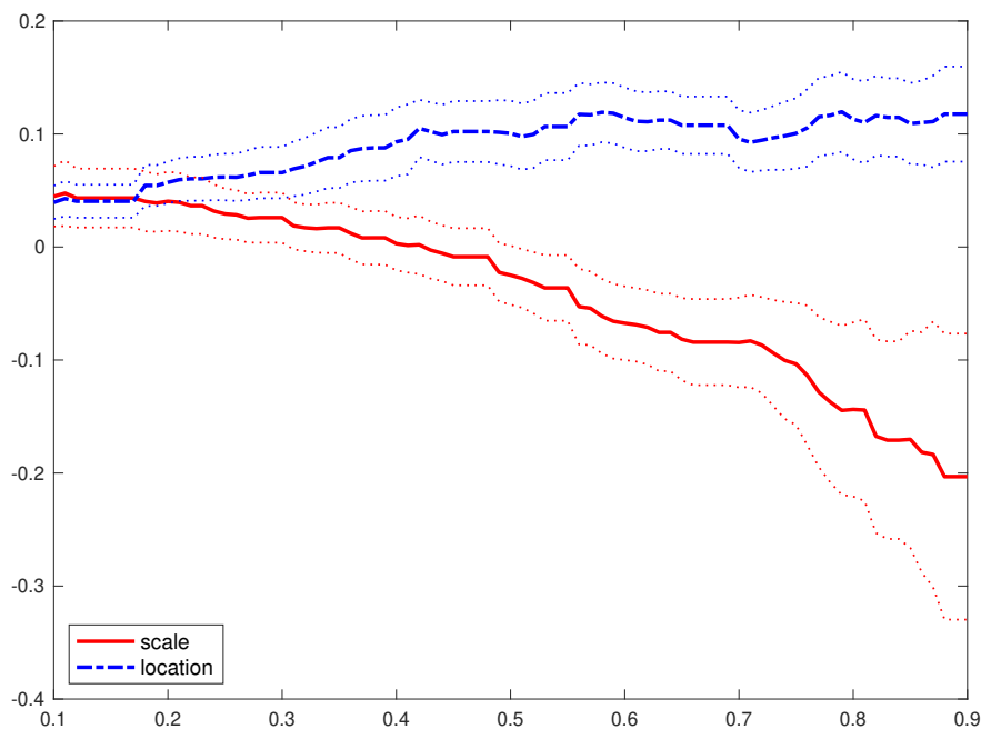
Figure 6: Point and interval estimates of location and scale effects of education on the unconditional quantiles of log-wage based on the probit specification: \Pi_{\tau,S} (solid red) and \Pi_{\tau,L} (dashed blue).
