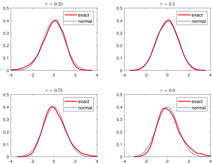
Figure 3: Finite sample exact distribution of the studentized scale effect statistic when \beta = 0.25 , \sigma_X^2 = 1 , and n = 1000 .
