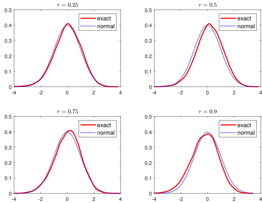
Figure 2: Finite sample exact distribution of the studentized location effect statistic when \beta = 0.75 , \sigma_X^2 = 1 , and n = 1000 .
