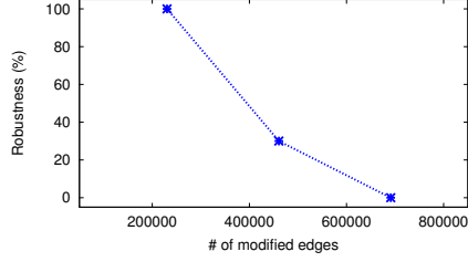
Figure 4.7: Robustness of the improved design against single attacker model, LA.
