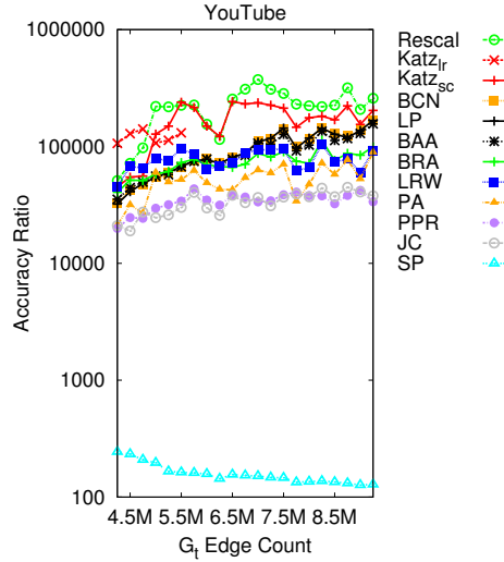
Figure 3.7: Link prediction performance for YouTube dataset. From Figure 3.5 to Figure 3.7 we show accuracy ratio of all metric-based prediction algorithms. We omit the results of CN, AA and RA because they perform similarly (slightly worse) than their Local Naive Bayes versions, i.e. BCN, BAA and BRA. The results for Katz lr in Renren and YouTube are capped to 65M and 5.5M edges due to computation complexity.
