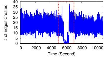
Figure 2.14: Examples of abnormal segments in terms of momentary outage , where the red dot boxes show the unusual edge creation events (sampled dataset of Renren).
