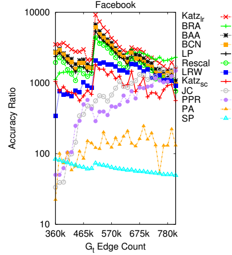
Figure 3.6: Link prediction performance for Facebook dataset.
