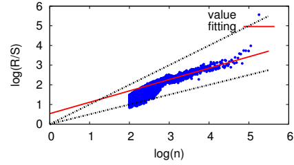
Figure 2.19: R/S analysis on the entire data: doubtful fitting since the shape changes greatly after 10^3 units (Facebook).
