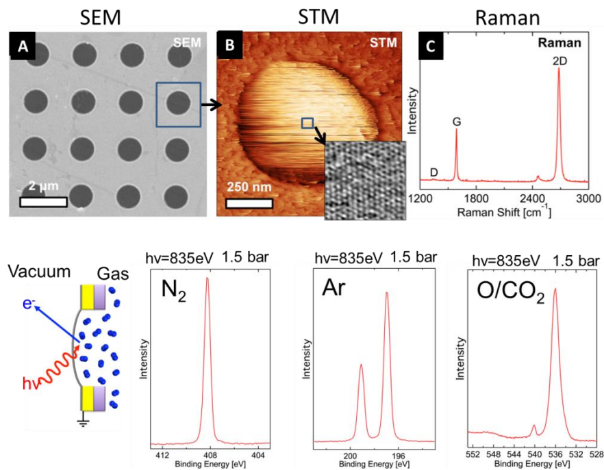
Fig. 4 . Top: A) SEM image of a holey \text{SiN} membrane (1 \mu\text{m} diameter) covered by a single layer graphene (SLG). B) STM image of one the holes in the membrane with SLG suspended across it. The inset shows an atomic resolution STM image of free-standing graphene. C) Raman spectra of SLG transferred onto \text{SiO}_2(300\text{ nm})/\text{Si} using the same method used for fabricating the graphene-based membranes. Bottom: Schematic of the XPS experiment, showing one of the holes and the SLG separating vacuum in the Synchrotron beam line on the left and gas on the right inside the cell. The pressure can reach up to 2.5 bar ( \sim\text{atm} ), depending on the quality and defects of the graphene. Three spectra are shown for \text{N}_2 , Ar and \text{CO}_2 on the right at 1.5 bar. Other gases are also possible ( \text{H}_2 , He, CO). The OK-level peak in \text{CO}_2 shows two peaks, one from the \text{CO}_2 gas molecules, the other at 540 eV from O bound to the graphene due to beam damage. Adapted from Ref. [22]. Copyright (2017) American Chemical Society.
