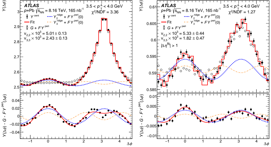
Figure 1: Template fitting output for events with jet p_T > 100 GeV. Both require 3.5 < p_T^A < 4.0 GeV and are made with 60–90% peripheral selection and 0–5% central selection. The left plot is made with no selection on the B-particles and the right plot is made requiring the B-particles to have |\Delta\eta^{Bj}| > 1 relative to all jets with p_T^{\text{jet}} > 15 GeV in the event. In the upper panels, the open circles show the scaled and shifted peripheral template with uncertainties omitted, the closed circles show the central data, and the red line shows the fit (template and harmonic functions). The blue dashed line shows the second-order harmonic component, Y_2^{\text{ridge}} , and the orange dotted line shows the third-order harmonic component, Y_3^{\text{ridge}} (the n = 2 and n = 3 contributions to the sum in Eq. 1, respectively). The lower panels show the difference between the central data and the peripheral template along with the second and third harmonic functions. The resulting v_{2,2} , v_{3,3} , and global fit \chi^2/\text{NDF} values are reported in the legends. In these fits, \text{NDF} = 35 .
