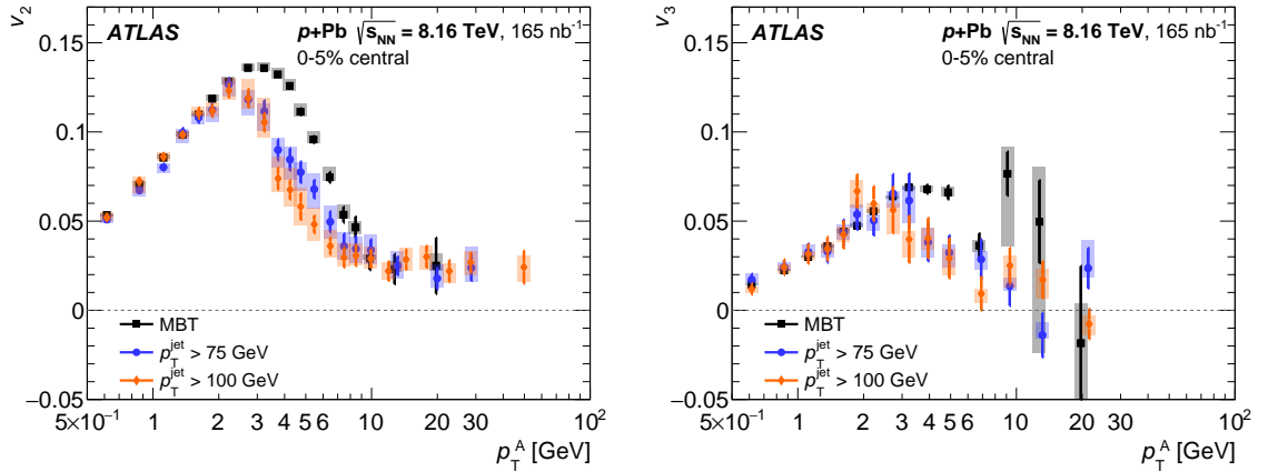
Figure 3: Distribution of v_2 (left) and v_3 (right) plotted as a function of the A-particle p_T . Values from MBT events are plotted as black squares, and those from events with jet p_T > 75 GeV and events with jet p_T > 100 GeV are plotted as blue circles and orange diamonds respectively. Statistical uncertainties are shown as narrow vertical lines on each point, and systematic uncertainties are presented as coloured boxes behind the points.
