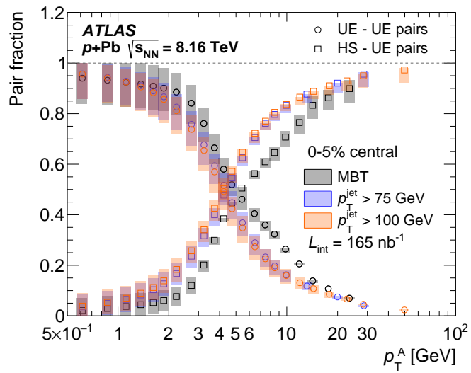
Figure 11: Underlying event–underlying event (UE–UE) (open circles) and hard scatter–underlying event (HS–UE) (open squares) particle-pair yield composition fractions for MBT events (black), events with jet p_T > 75 GeV (blue), and events with jet p_T > 100 GeV (orange) plotted as a function of the A-particle p_T . Statistical uncertainties are shown as narrow vertical lines on each point, and systematic uncertainties are presented as coloured boxes behind the points.
