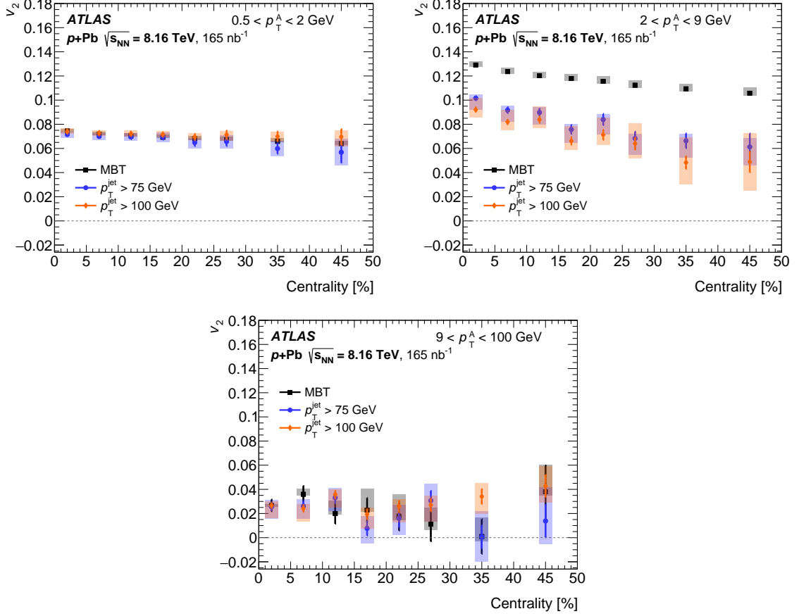
Figure 5: Distribution of v_2 plotted as a function of centrality for MBT events (black squares), events with jet p_T > 75 GeV (blue circles), and events with jet p_T > 100 GeV (orange diamonds). The results are obtained in three different selections of the A-particle p_T : 0.5 < p_T < 2 GeV (top left), 2 < p_T < 9 GeV (top right), and 9 < p_T < 100 GeV (bottom). Statistical uncertainties are shown as narrow vertical lines on each point, and systematic uncertainties are presented as coloured boxes behind the points.
