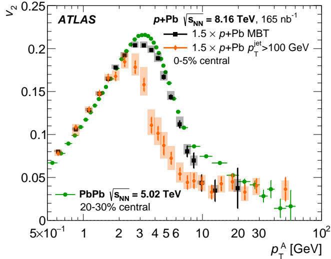
Figure 9: Scaled p +Pb v_2 values plotted as a function of the A-particle p_T overlaid with v_2 from 20–30% central Pb+Pb data at \sqrt{s_{NN}} = 5.02 TeV [62]. Results from MBT and jet p_T > 100 GeV p +Pb events are plotted as black squares and orange diamonds, respectively, and those from Pb+Pb are plotted as green circles. Statistical uncertainties are shown as narrow vertical lines on each point, and systematic uncertainties are presented as coloured boxes behind the points.
