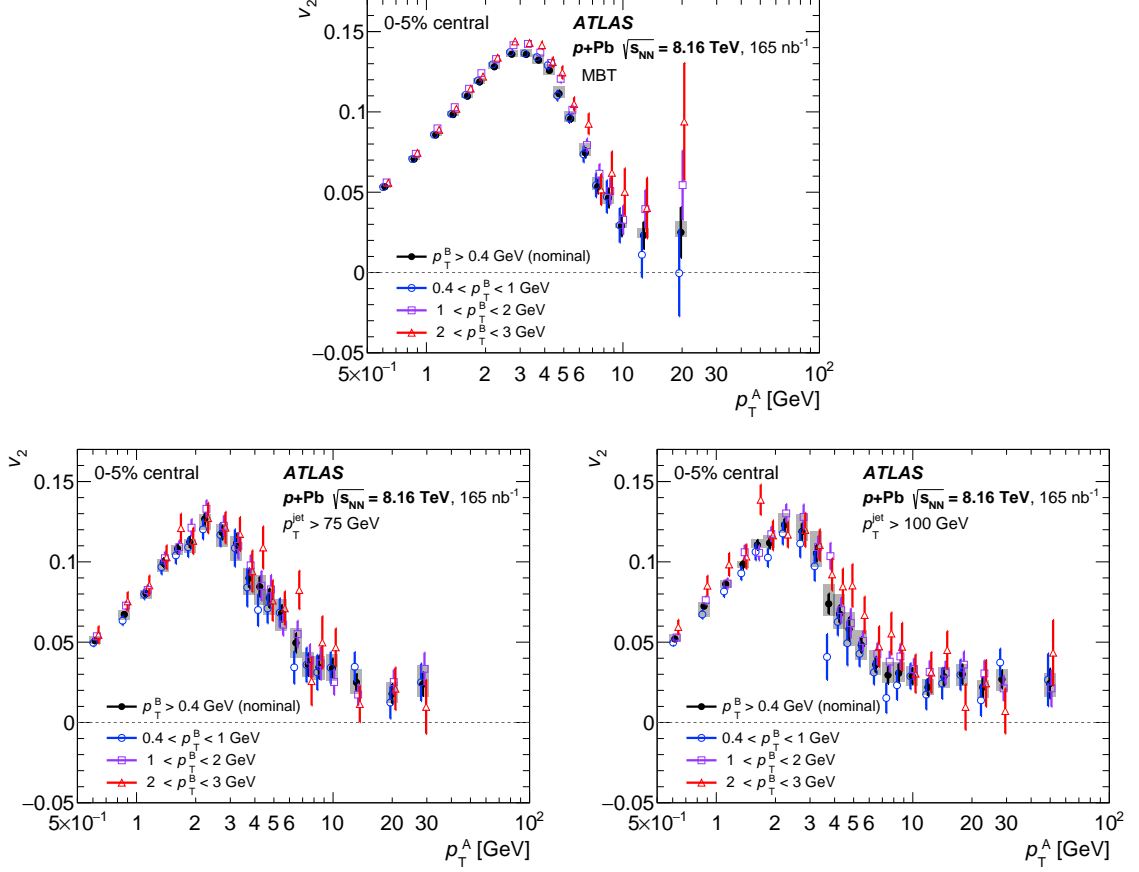
Figure 4: Measured v_2 values plotted as a function of the A-particle p_T for MBT events (top), events with jet p_T > 75 GeV (bottom left), and events with jet p_T > 100 GeV (bottom right). The nominal values (closed black circles) are overlaid with points generated by making different B-particle p_T selections: 0.4 < p_T^B < 1 GeV (blue open circles), 1 < p_T^B < 2 GeV (open violet squares), and 2 < p_T^B < 3 GeV (open red triangles). The points with different B-particle p_T selections are offset slightly from the nominal horizontal-axis positions to make the uncertainties visible.
