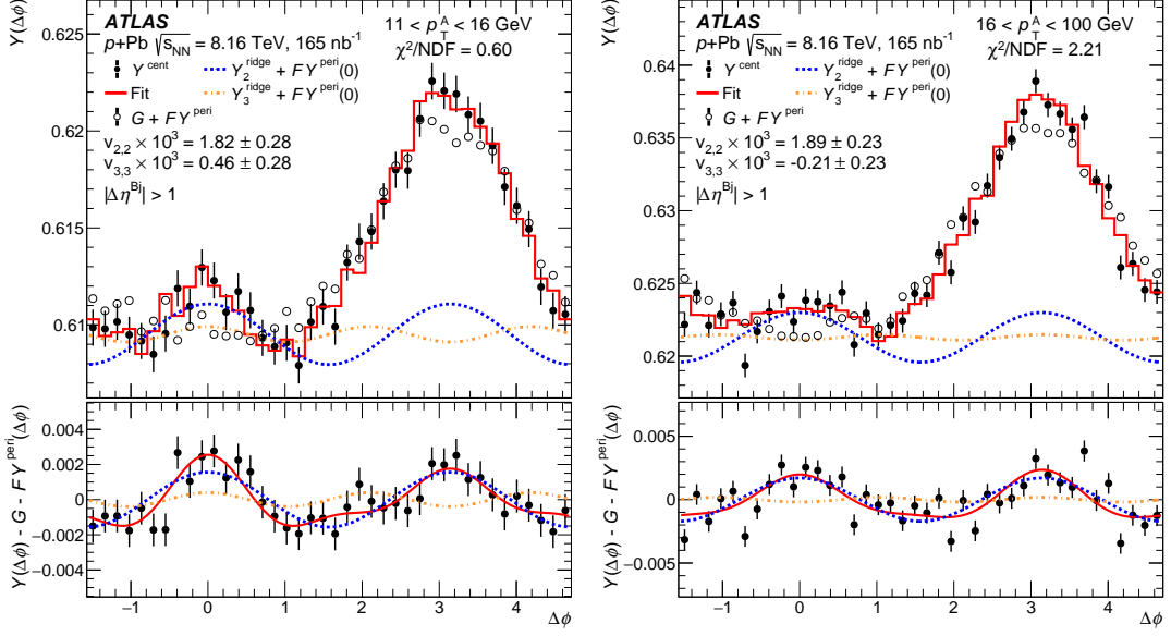
Figure 2: Template fitting output for events with jet p_T > 100 GeV with 60–90% peripheral selection and 0–5% central selection. The left plot is made with 11 < p_T^A < 16 GeV and the right plot with 16 < p_T^A < 100 GeV. In the upper panels, the open circles show the scaled and shifted peripheral template with uncertainties omitted, the closed circles show the central data, and the red line shows the fit (template and harmonic functions). The blue dashed line shows the second-order harmonic component, Y_2^{\text{ridge}} , and the orange dotted line shows the third-order harmonic component, Y_3^{\text{ridge}} (the n = 2 and n = 3 contributions to the sum in Eq. 1, respectively). The lower panels show the difference between the central data and the peripheral template along with the second and third harmonic functions. The resulting v_{2,2} , v_{3,3} , and global fit \chi^2/\text{NDF} values are reported in the legends. In these fits, \text{NDF} = 35 .
