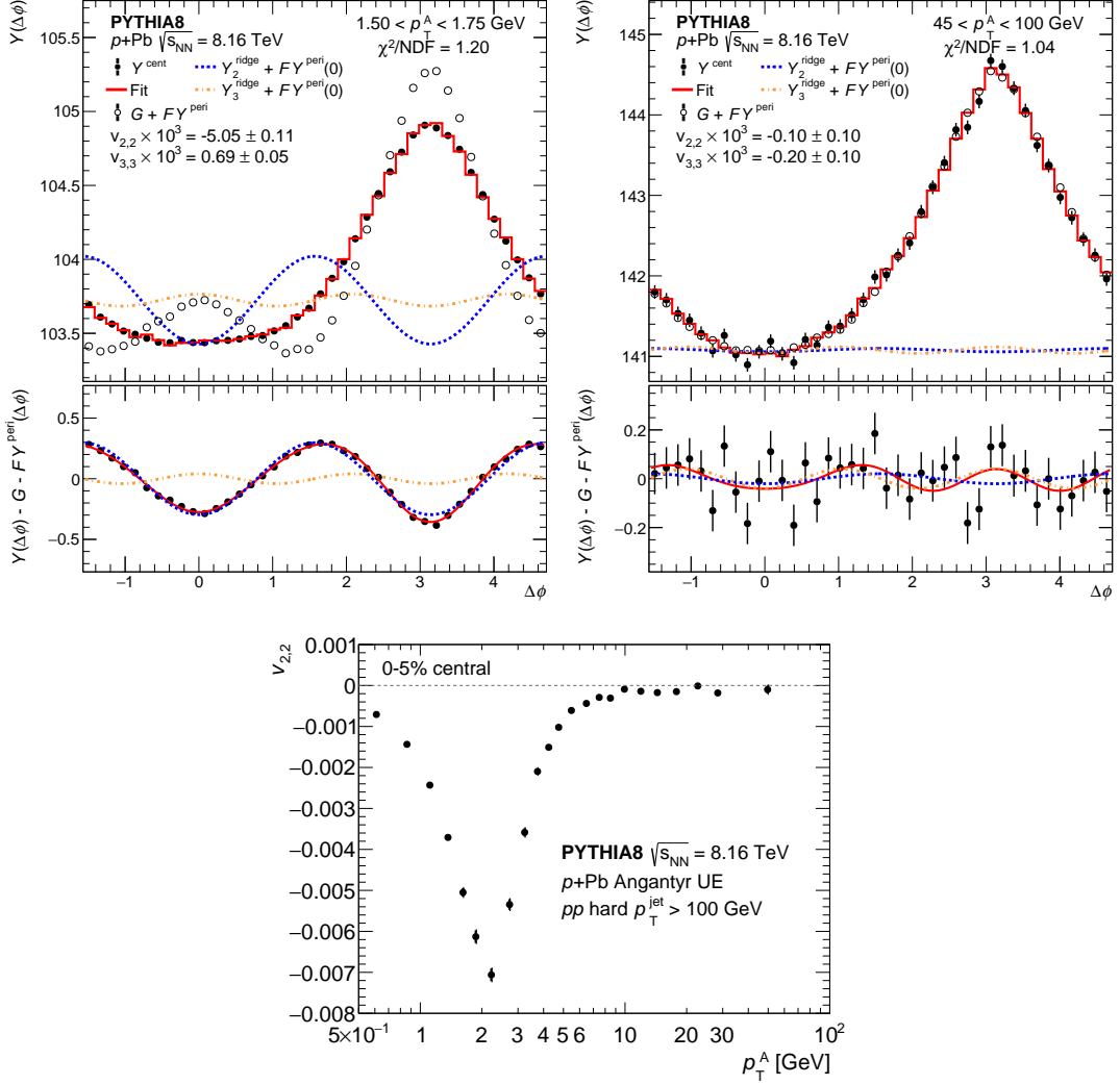
Figure 8: Predictions of azimuthal anisotropy from PYTHIA 8 using the same two-particle formalism used for the data results. The events combine minimum-bias p +Pb underlying events generated in the Angantyr framework with hard pp events that require the presence of a jet with p_T > 100 GeV. The two top plots show example correlation functions, with template fits, from a low particle- p_T selection (top left) and a high particle- p_T selection (top right). In the upper panels of the two top plots, the open circles show the scaled and shifted peripheral template with uncertainties omitted, the closed circles show the central data, and the red histogram shows the fit (template and harmonic functions). The blue dashed line shows the second-order harmonic component, Y_2^{\text{ridge}} , and the orange dashed line shows the third-order harmonic component, Y_3^{\text{ridge}} (the n = 2 and n = 3 contributions to the sum in Eq. 1, respectively). The lower panels show the difference between the central data and the peripheral template along with the second and third harmonic functions. The resulting v_{2,2} , v_{3,3} , and global fit \chi^2/\text{NDF} values are reported in the legends, where \text{NDF} = 35 . The bottom plot shows the extracted v_{2,2} values as a function of A-particle p_T .
