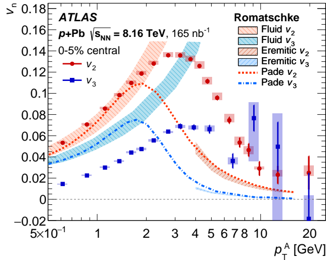
Figure 7: Coefficients v_2 and v_3 plotted as a function of p_T for central 0–5% p +Pb collisions from the MBT event sample. Theoretical calculations relevant to the low- p_T regime from hydrodynamics and to the high- p_T regime from an ‘eremitic’ framework from Romatschke [26] are also shown. The lines are Padé-type fits connecting the two regimes, where the red dotted line is for v_2 and the blue dash-dotted line is for v_3 . Statistical uncertainties are shown as narrow vertical lines on each point, and systematic uncertainties are presented as coloured boxes behind the points.
