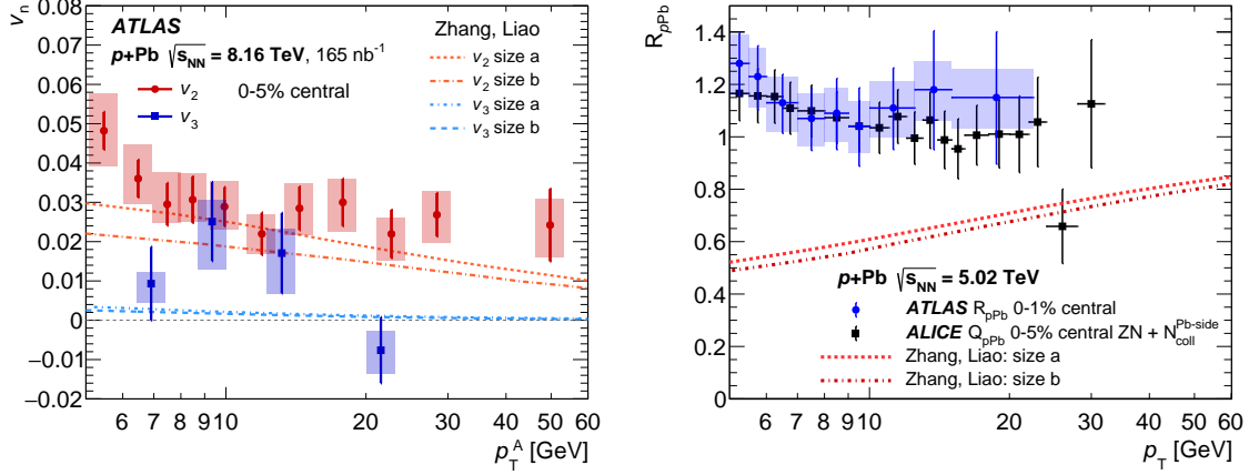
Figure 6: Coefficients v_2 and v_3 (left panel) and R_{pPb} (right panel) plotted as a function of particle p_T for p+Pb collisions. The left panel is for central 0–5% events from the jet p_T > 100 GeV event sample. Statistical uncertainties are shown as narrow vertical lines on each point, and systematic uncertainties are presented as coloured boxes behind the points. The left panel has two sets of curves showing theoretical predictions from a jet quenching framework with two different initial geometries in 0–4% central collisions [14]; the upper two (red/orange) are v_2 for ‘size a’ (dotted) and ‘size b’ (dash-dotted) configurations, and the lower two (blue) are v_3 where the ‘size a’ (dash-dotted) and ‘size b’ (dashed) curves are nearly indistinguishable from each other. The right panel shows R_{pPb} data from ATLAS [57] and Q_{pPb} data from ALICE [41]. Theoretical calculations (red/orange lines) from Ref. [14] are also shown in this panel; the dotted line gives the results of the ‘size a’ configuration and the dash-dotted line gives the results of the ‘size b’ configuration.
