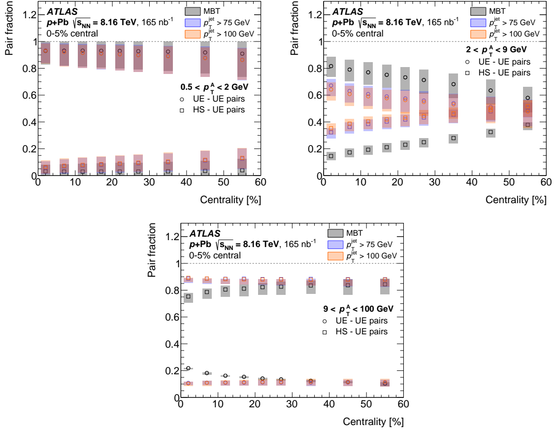
Figure 12: Underlying event–underlying event (UE–UE) (open circles) and hard scatter–underlying event (HS–UE) (open squares) particle–pair yield composition fractions for MBT events (black), events with jet p_T > 75 GeV (blue), and events with jet p_T > 100 GeV (orange) plotted as a function of event centrality. The results are obtained in three different selections of the A-particle p_T : 0.5 < p_T < 2 GeV (top left), 2 < p_T < 9 GeV (top right), and 9 < p_T < 100 GeV (bottom). Statistical uncertainties are shown as narrow vertical lines on each point, and systematic uncertainties are presented as coloured boxes behind the points.
