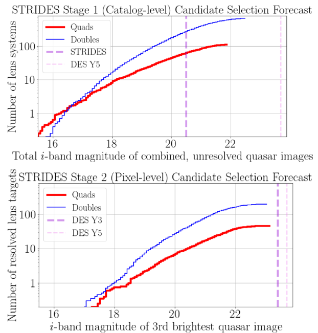
Figure 1. Cumulative number of expected lensed quasars for STRIDES based on the Oguri & Marshall (2010) catalogue, in an approximate emulation of the STRIDES lens selection. Thick solid red lines represent quads, thin solid blue lines represent doubles. Top: expected number of lenses in the DES+ WISE catalogues, as a function of total lensed quasar magnitude. Bottom: expected number of catalogue-selected lenses visible (i.e. resolved as lenses, with detectable counter-images) in the DES images.
