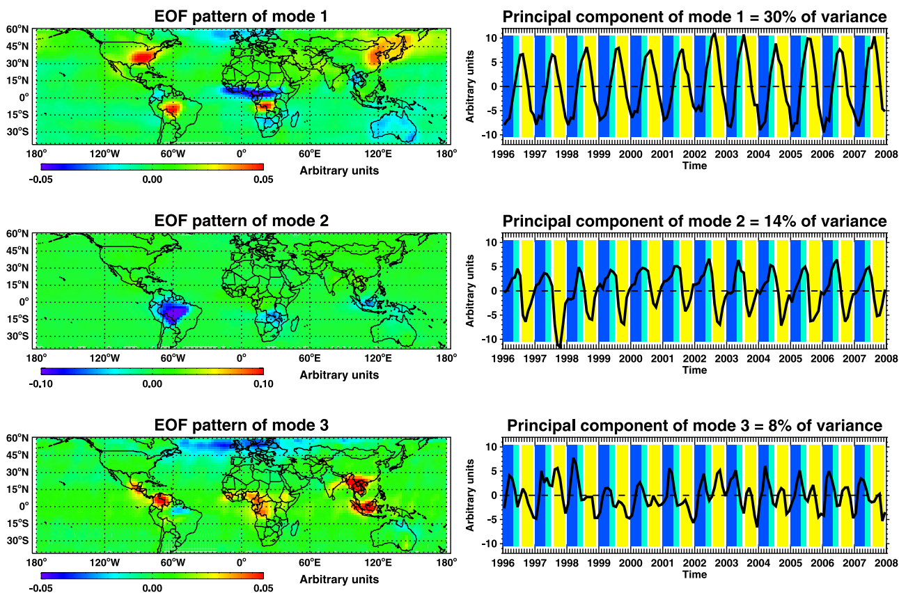
Figure 1. The first three eigenvectors of the Empirical Orthogonal Function (EOF) analysis of the monthly HCHO column distributions averaged on to 2^\circ \times 2.5^\circ (latitude \times longitude) grid, excluding scenes with >40\% cloud coverage. The (left) EOF regression maps and (right) principal components with their corresponding eigenvalues show the dominant spatial and temporal variations of the HCHO columns, respectively. The dark blue, light blue, and yellow regions shown on the principal components represent the wet (January–April), transition (May–June), and dry (August–November) seasons over the Amazon [Barkley et al. , 2008], respectively.
