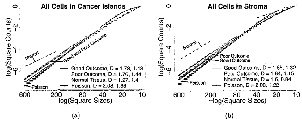
Fig. 6. Log-log plot of the number of squares with at least one cell (of any type) that is in (a) a cancer cell island or epithelial tissue or (b) in the stroma versus the inverse box size in microns. (a) At long length scales (200–600 microns on the left side of plot), the mean fractal dimension x (slope) is 1.78 for good outcome (dark, solid), 1.76 for poor outcome (light, dashed), 1.27 for normal tissue (light, solid) and 2.08 for Poisson (black). The p -value for good versus poor outcome is 0.57 for long length scales. At short length scales (10–40 microns), the mean fractal dimension x (slope) is 1.48 for good outcome (dark, solid), 1.44 for poor outcome (light, dashed), 1.4 for normal tissue (light, solid) and 1.36 for Poisson (black). The p -value for good versus poor outcome is 0.49 at short length scales. (b) At long length scales (200–600 microns on the left side of plot), the mean fractal dimension x (slope) is 1.85 for good outcome (dark, solid), 1.84 for poor outcome (light, dashed), 1.6 for normal tissue (light, solid) and 2.08 for Poisson (black). The p -value for good versus poor outcome is 0.64 for long length scales. At short length scales (10–40 microns), the mean fractal dimension x (slope) is 1.32 for good outcome (dark, solid), 1.15 for poor outcome (light, dashed), 0.84 for normal tissue (light, solid) and 1.22 for Poisson (black). The p -value for good versus poor outcome is 0.013 for short length scales. Black dashed lines show the least squares linear regression fit at long and short length scales. Because different images had different numbers of squares with tissue (cells of any type), for each image, we normalized the number n(L) of boxes with 1's by the total number N(L) of boxes with cells in computing the fractal dimension. Thus, the y -axis values are negative. The error bars correspond to 95% confidence intervals.
