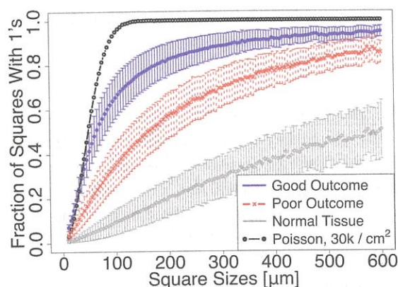
Fig. 2. Plot of CD8 + T cell occupancy versus square size for good clinical outcome (blue, solid), poor clinical outcome (red, dashed) and points randomly distributed according to a uniform Poisson process with a density of 3 \times 10^4 points/cm 2 (solid black line). The error bars indicate 95% confidence intervals. 1,2
