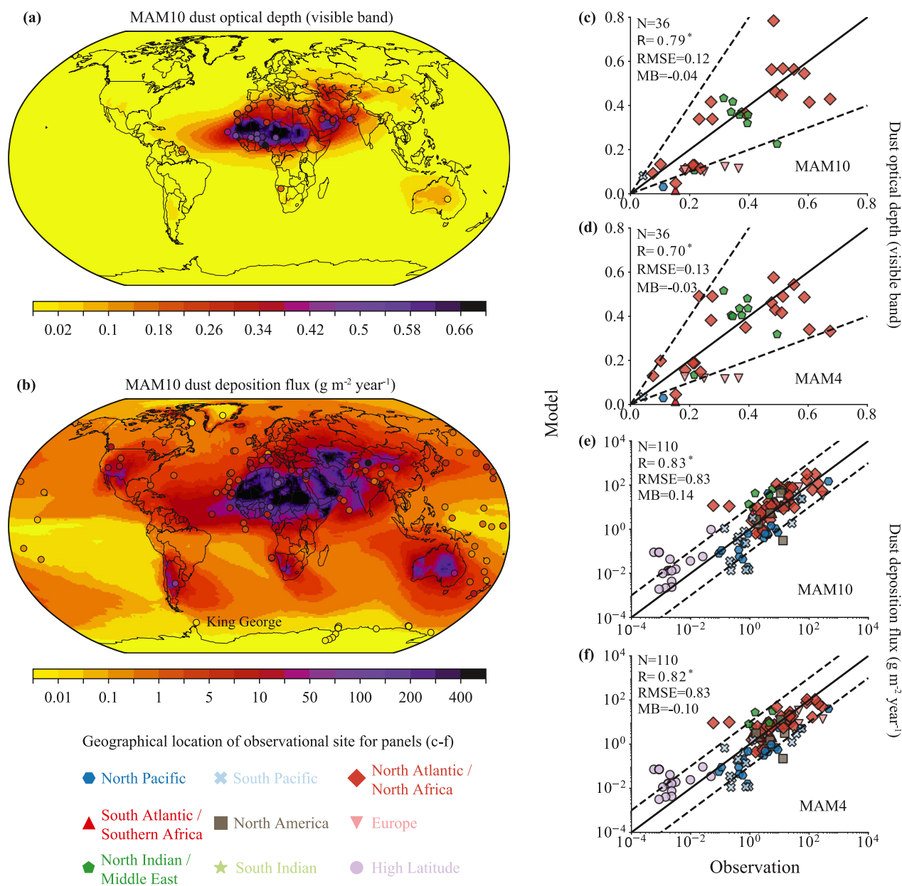
Figure 1. Comparison of simulated total dust quantities with observational data (total number: N) previously compiled (Albani et al., 2014). Panels (a), (c), and (d) show dust optical depth in the 0.44–0.63 \mu\text{m} band, while panels (b), (e), and (f) present deposition fluxes. The deposition fluxes represent values for dust particles with geometric diameters smaller than 10 \mu\text{m} . Black solid lines in scatter plots indicate the one-one line, and dashed lines show a factor of 2.0 (panels c and d) or 10 (panels e and f) difference. Model (MAM10: panels a–c, and e; MAM4: panels d and f) performance metrics include Pearson's correlation (R; “*” indicates significance at the 95% confidence level), root mean square error (RMSE; same units as the corresponding dust quantities), and mean bias (MB; same units as the corresponding dust quantities), calculated in the logarithmic space for deposition fluxes and in the normal space for dust optical depth. Table S1 in Supporting Information S1 provides the definition of the geographical regions.
