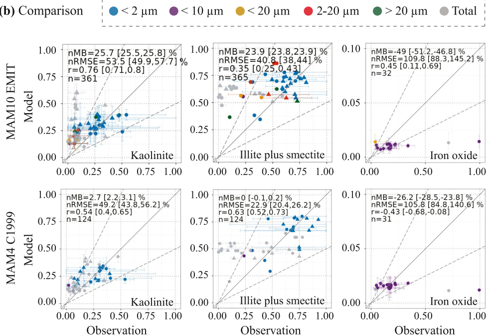
Figure 7. Mineral sample locations and model-simulated mineral fractions in surface concentrations or deposition, compared to previously compiled observations (total number: n ) (Perlwitz et al., 2015a, 2015b) using the approach of Gonçalves Ageitos et al. (2023). (a) Mineral sample locations categorized by geophysical zones, obtained from surface concentrations (red circles), dry deposition (green squares), or total deposition (green triangles). (b) Model-observation comparisons for kaolinite, smectite, and iron oxides across different size (geometric diameter) segments: top panels for MAM10 with the EMIT soil atlas and bottom panels for MAM4 with the Claquin et al. (1999) soil atlas (C1999). Model performance is evaluated using normalized mean bias (nMB; in percentage), normalized root mean square error (nRMSE; in percentage), and size and spatial correlation ( r ), based on different sample sizes ( n : number of observational samples used in each plot). See Figure S7 in Supporting Information S1 for the other minerals.
