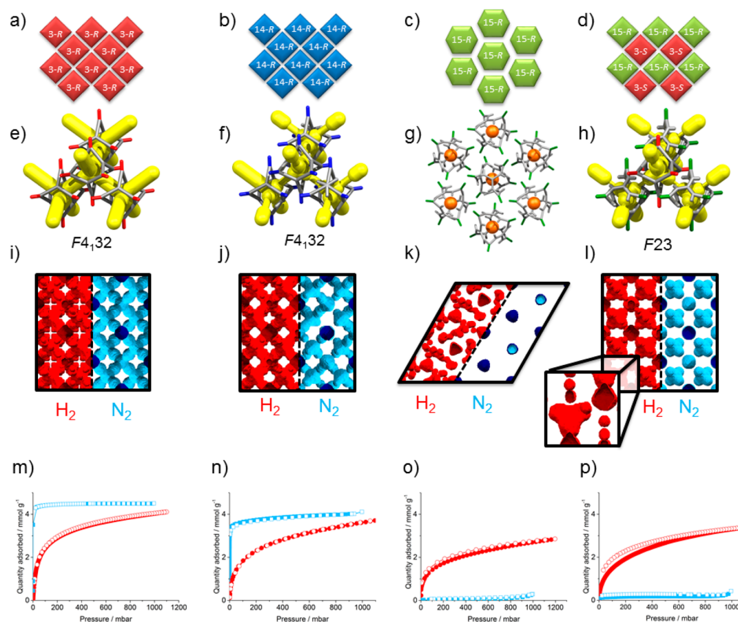
Figure 2. Crystal packing, pore topology, surface area plots, and sorption isotherms for homochiral CC3\alpha , CC14\alpha , CC15\alpha , and CC3-S/CC15-R cocrystal. (a–d) Simplified representation of the cage packing in CC3\alpha , CC14\alpha , CC15\alpha , and CC3-S/CC15-R cocrystal. (e–h) Simplified representation of the crystal structures of these cages, with pore channels shown in yellow. (i–l) Surface area plots, measured with two probe sizes: H_2 (red, 1.09 Å) and N_2 (blue, 1.7 Å). As more methyl groups are added to the structures (from left to right), the pores become narrower; in CC15\alpha and CC3-S/CC15-R cocrystal the cage cavities are occluded for a N_2 probe. These correlate well with the (m–p) hydrogen (red) and nitrogen (blue) sorption isotherms for CC3\alpha , CC14\alpha , CC15\alpha , and CC3-S/CC15-R cocrystal respectively at 77 K and 1 bar. Closed symbols show adsorption, and open symbols show desorption isotherms, respectively.
