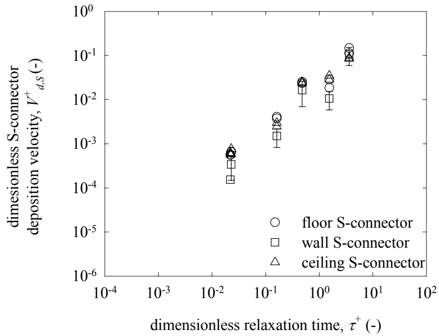
Figure 4.2 Dimensionless deposition velocities to S-connectors on the ceiling, wall and floor at an air speed of 5.3 m/s.
