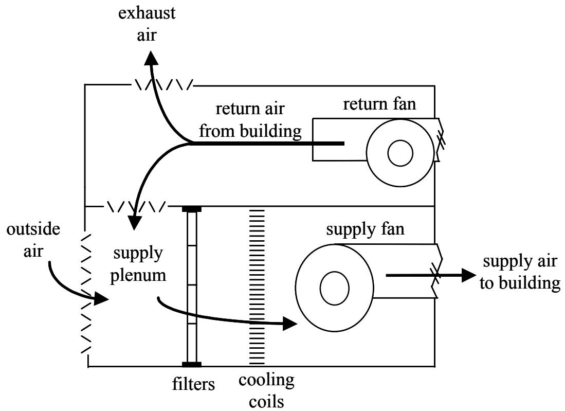
Figure 1.1 Schematic diagram of airflow through the mechanical room for a typical HVAC system.
