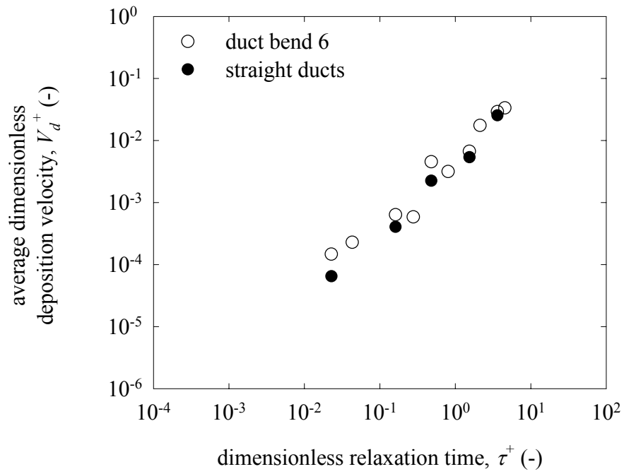
Figure 4.13 Composite dimensionless deposition velocities in bend 6 and in test ducts 1 and 2 versus dimensionless relaxation time at an air speed of 5.3 m/s.
