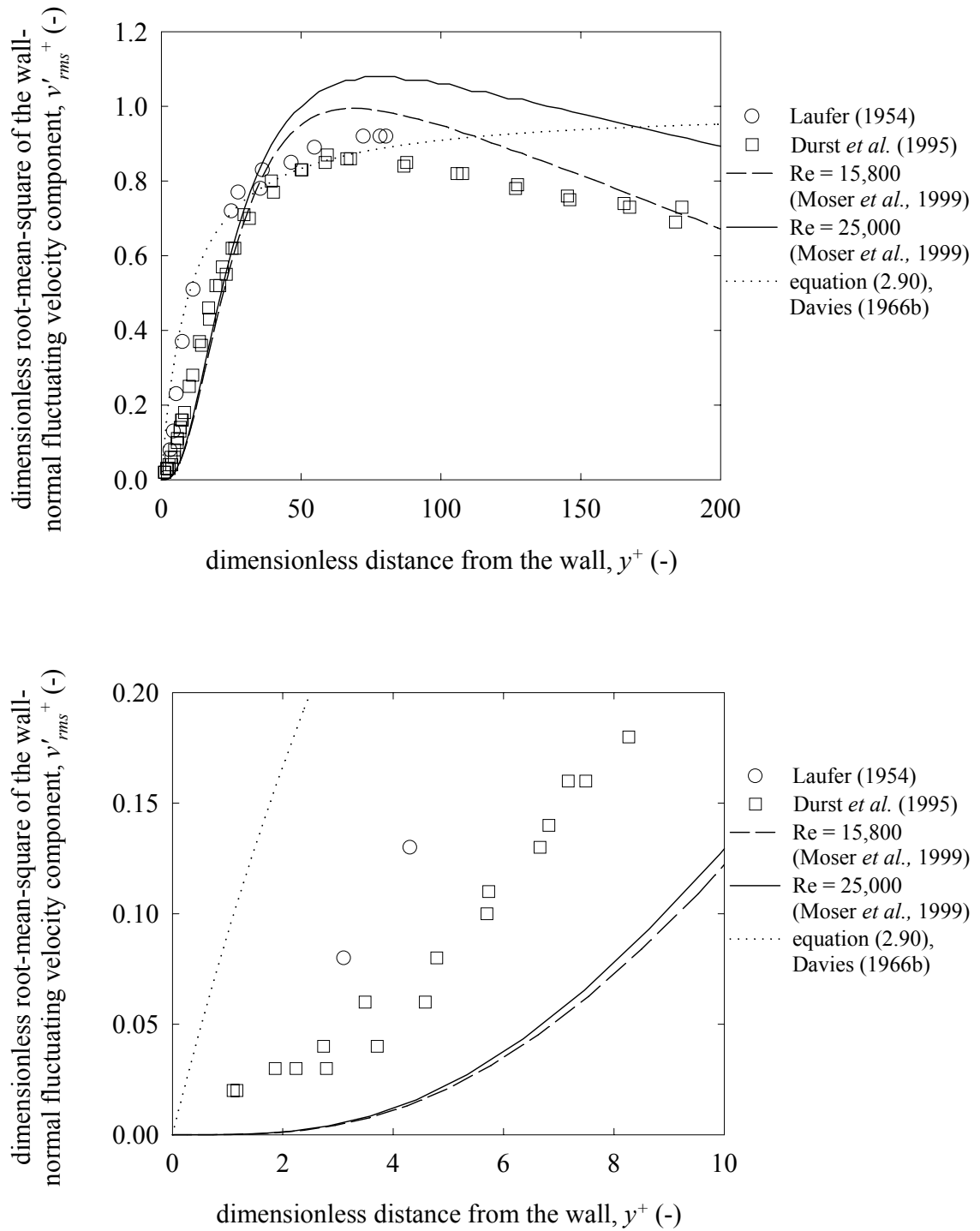
Figure 2.11 Profiles of v'_{rms}+ versus y^+ derived from measurements in pipe flow and DNS of channel flow. The bottom panel shows the same data as the top panel with the axes scaled to focus attention near the wall.
