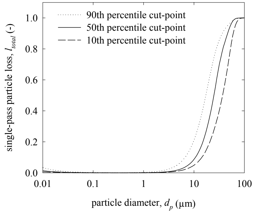
Figure 6.3 Predicted fractional losses for a single pass through return duct runs.
