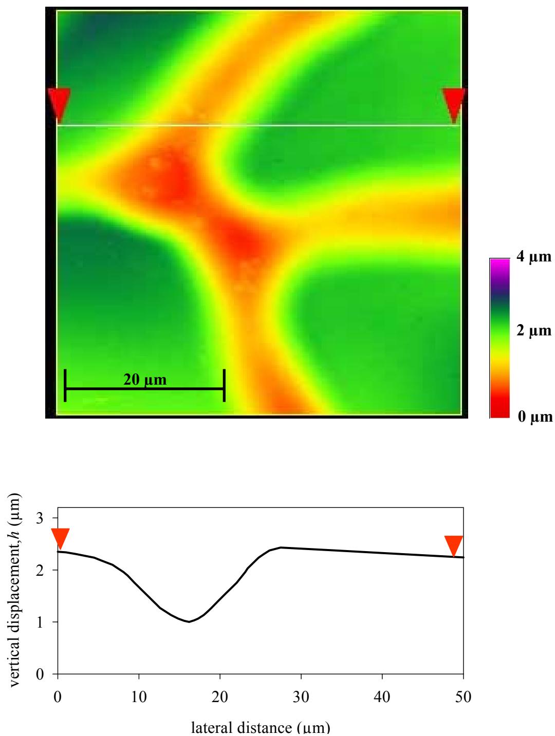
Figure A.4 Two-dimensional contour plot of the surface of a steel experimental duct from an atomic force microscope. The lower panel displays a plot of the surface height versus the lateral distance for the section through the surface demarked by the pointers.
