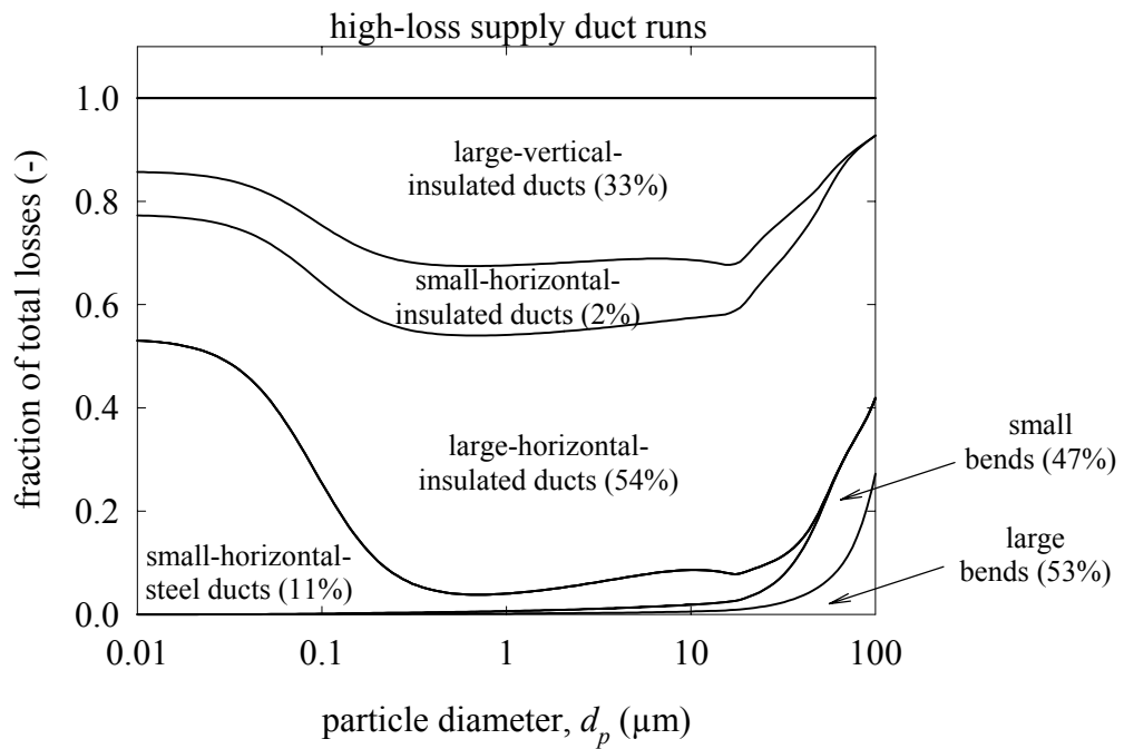
6.9 Fraction of total losses occurring in different duct generation classes for low-loss and high-loss supply duct runs.
