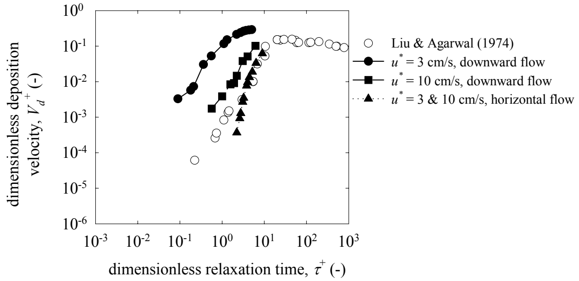
Figure 2.44 Deposition to a smooth vertical wall in the DNS-Lagrangian simulation of Zhang & Ahmadi (2000) with downward and horizontal flow at low friction velocities compared to the experiments of Liu & Agarwal (1974).
