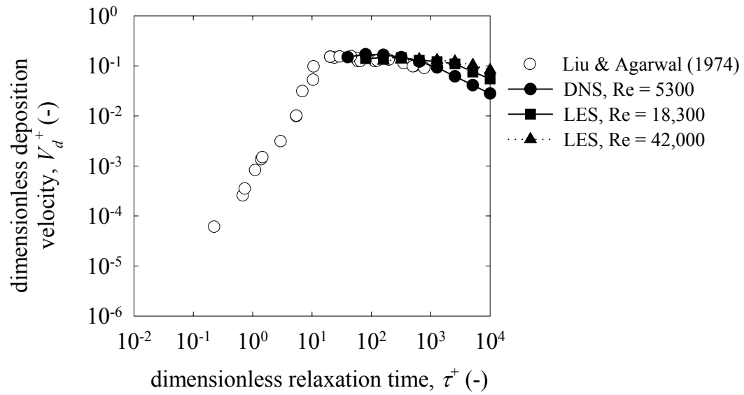
Figure 2.42 Deposition to smooth vertical walls in the DNS- and LES-Lagrangian simulations of Uijttewaai & Oliemans (1996) compared to the experiments of Liu & Agarwal (1974).
