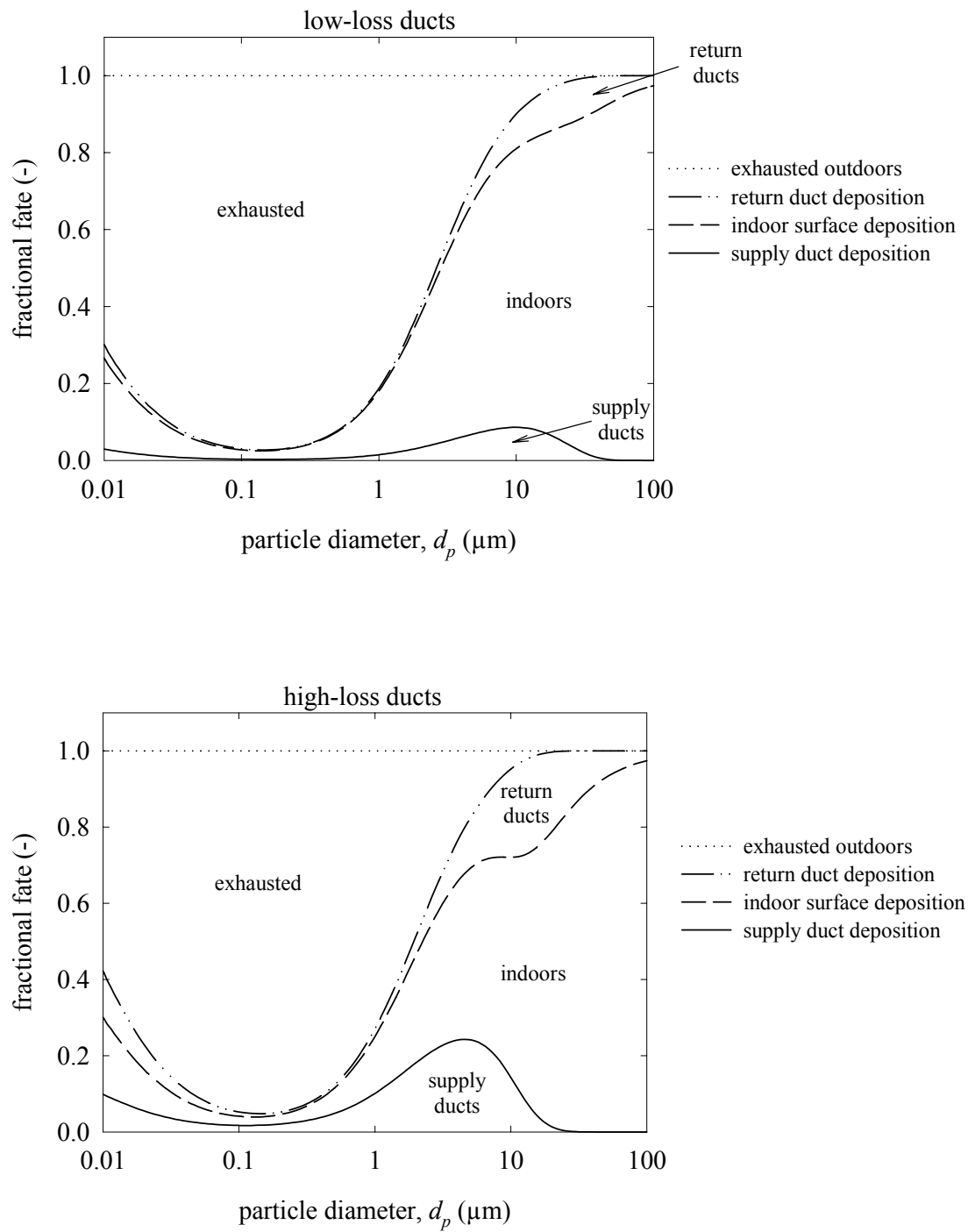
Figure 6.16 Predicted fractional fates of particles released in a building with an unfiltered ventilation system for both low-loss and high-loss ducts.
