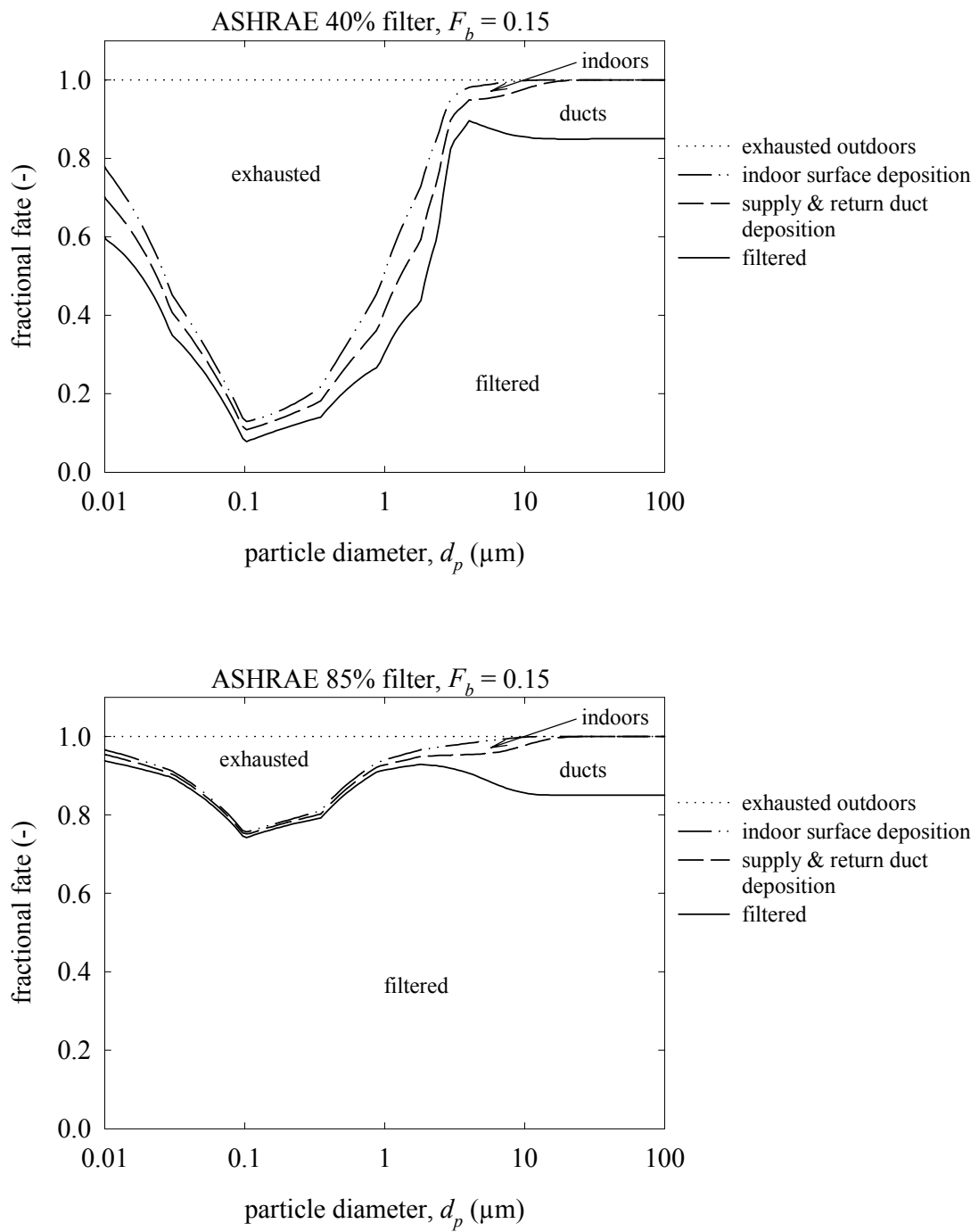
Figure 6.13 Predicted fractional fates of outdoor particles drawn into air intakes with either ASHRAE 40% or ASHRAE 85% efficient filters and a filter bypass fraction, F_b , of 0.15 for high-loss ducts.
