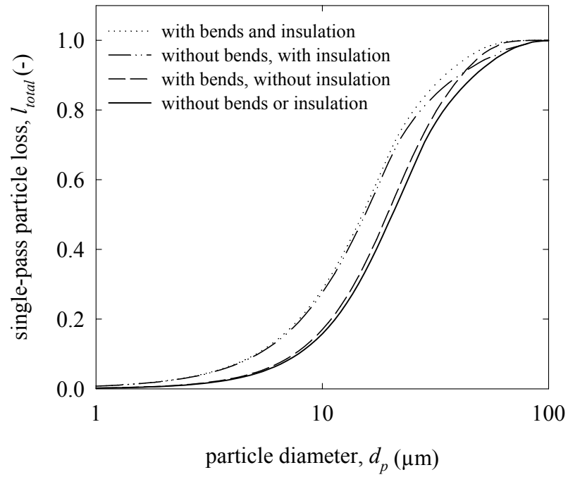
Figure 6.5 Predicted fractional losses in a medium-loss duct run considering the influence of duct bends and interior insulation.
