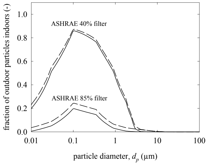
Figure 6.15 Predicted fraction of outdoor particles remaining indoors for particles drawn into an air intake with ASHRAE 40% filters and a bypass fraction, F_b , of zero or 0.15 for ducts with average losses.
