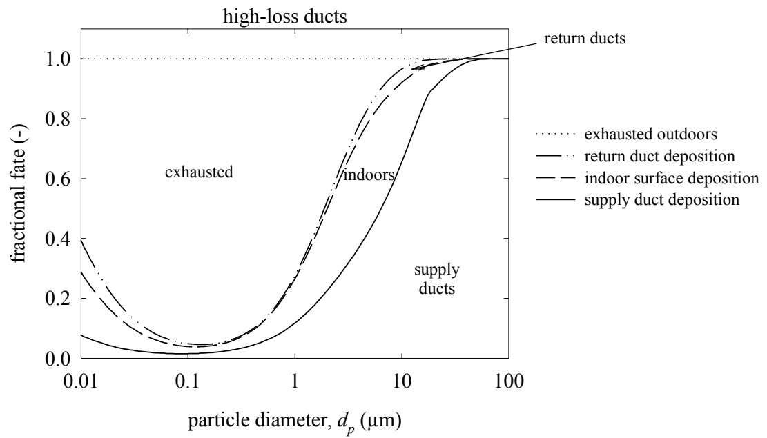
Figure 6.10 Predicted fractional fates of outdoor particles drawn into an unfiltered air intake for low-loss and high-loss ducts.
