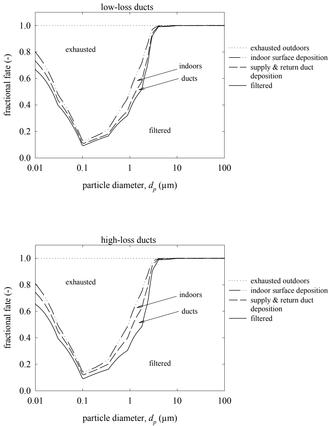
Figure 6.11 Predicted fractional fates of outdoor particles drawn into an air intake with ASHRAE 40% efficient filters for low-loss and high-loss ducts.
