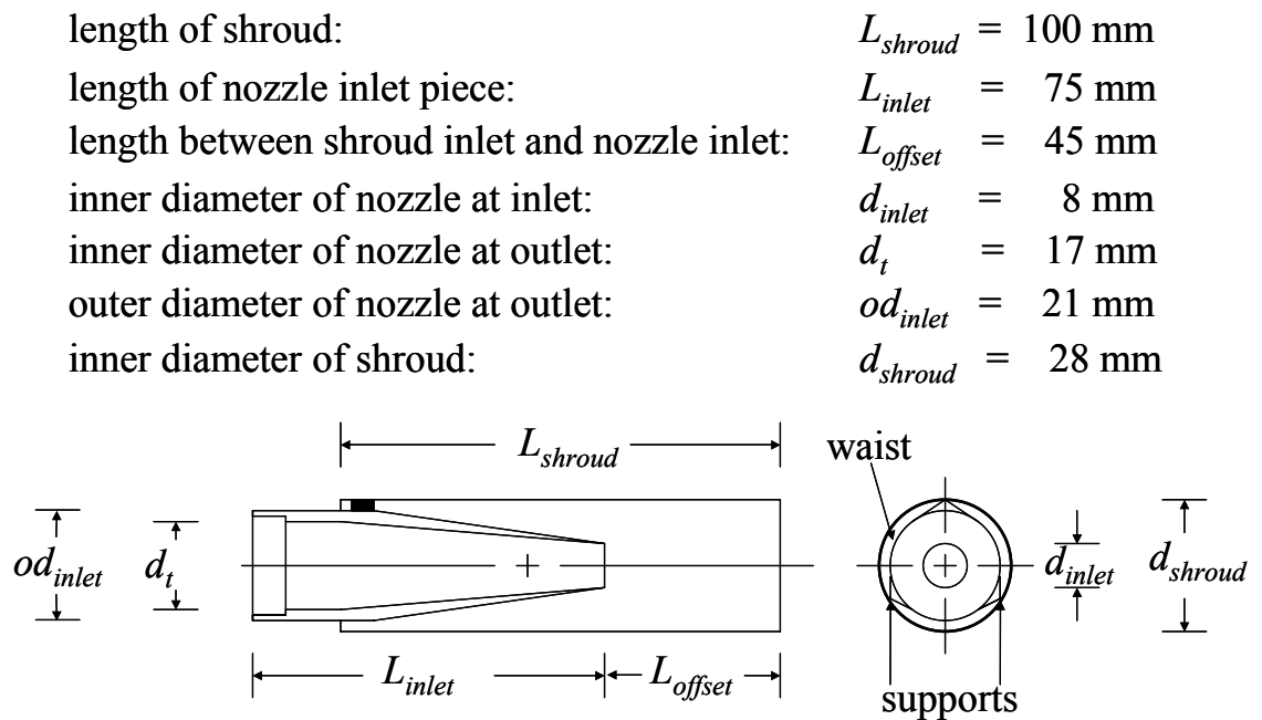
Figure B.4 Schematics of a side view of a section through the centerline of the shrouded inlet and of an end view of the inlet. Dimensions of defined parameters are also given.
