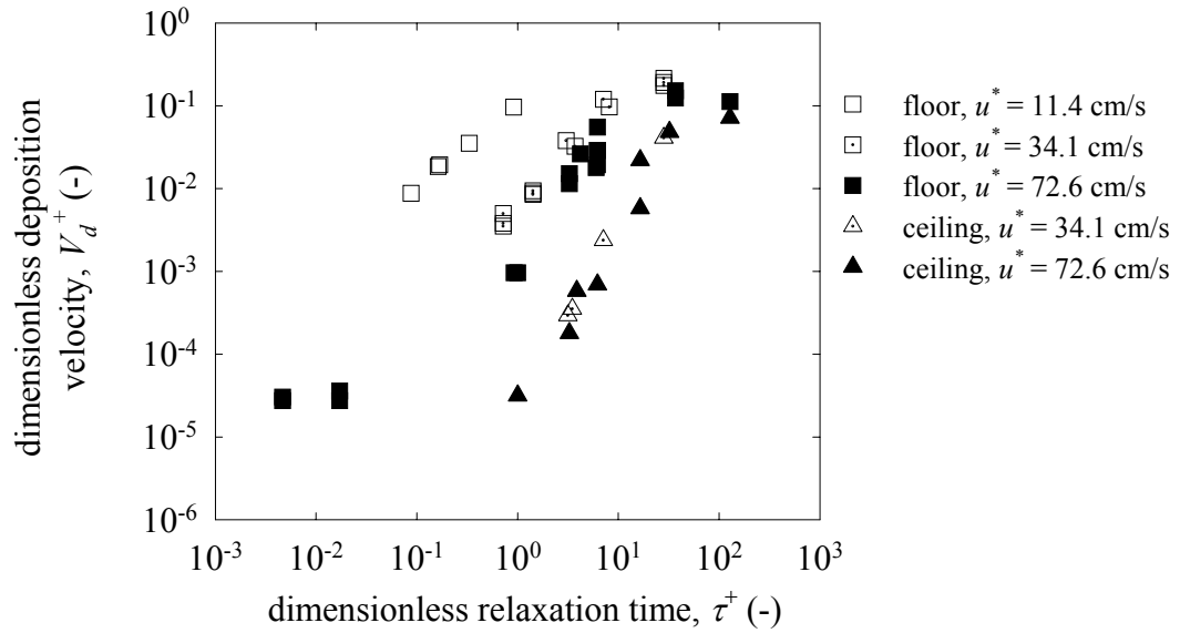
Figure 2.8 Experimental data collected by Sehmel (1973) for deposition to the smooth floor and ceiling of a horizontal duct at three different values of the friction velocity, u^* .
