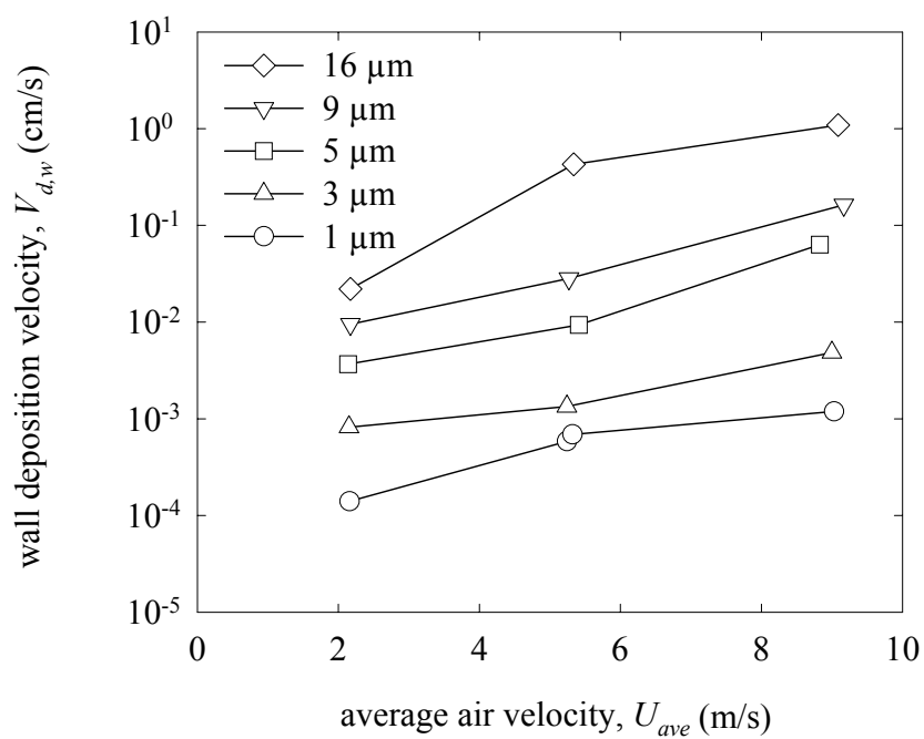
Figure 3.9 Average measured deposition velocity to the wall of test ducts 1 and 2 versus air speed in the steel system.
