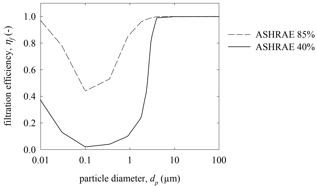
Figure 6.2 Filtration efficiency of ASHRAE 40% and ASHRAE 85% filters.
