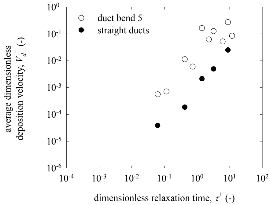
Figure 4.11 Composite dimensionless deposition velocities in bend 5 and in test ducts 1 and 2 versus dimensionless relaxation time at an air speed of 9.0 m/s.
