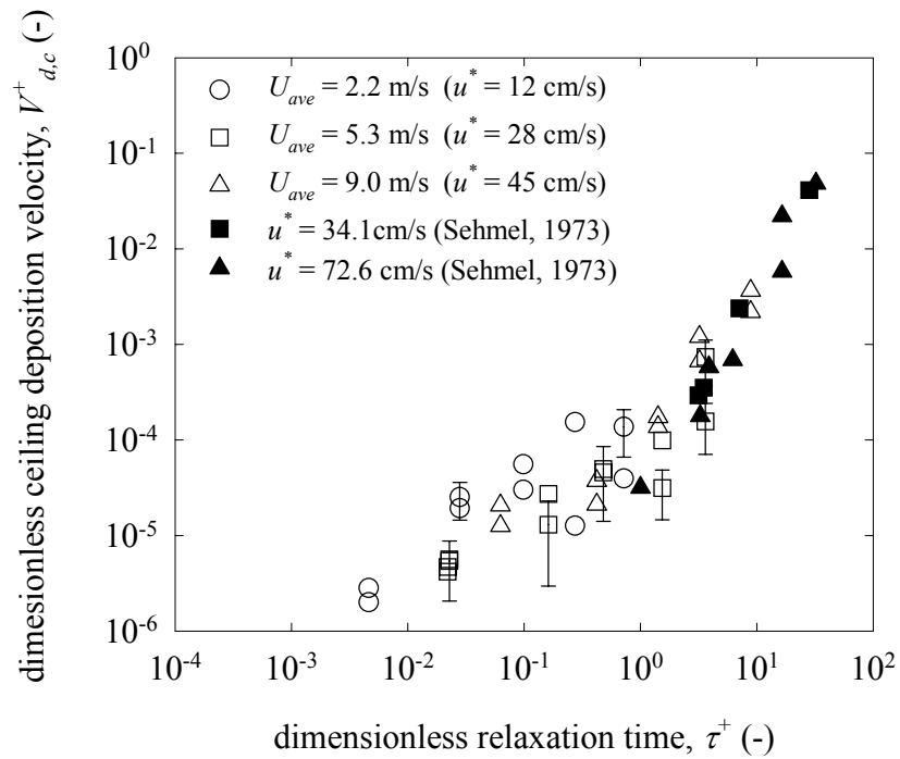
Figure 3.15 Comparison of dimensionless ceiling deposition velocities measured at three air speeds in the steel system with the data of Sehmel (1973).
