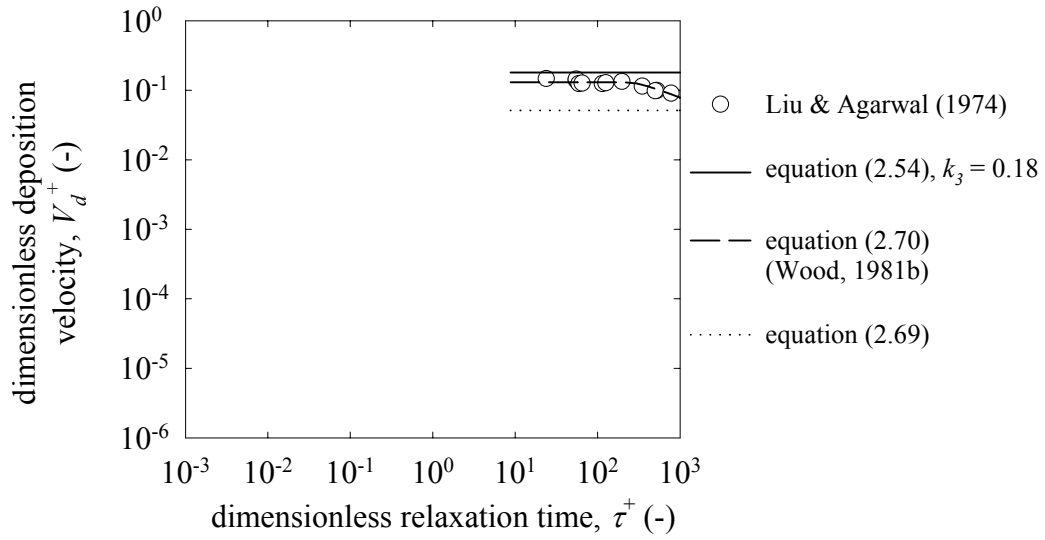
Figure 2.20 Comparison of empirical expressions for deposition to smooth vertical walls in the inertia-moderated regime.
