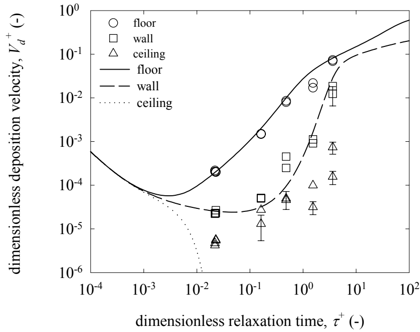
Figure 5.20 Comparison of the turbophoretic model of Guha (1997) with a roughness of 5 \mu\text{m} , an air-wall \Delta T of 0.2^\circ\text{C} and equation (5.2) for v_{rms}^+ to data collected in steel ducts.
