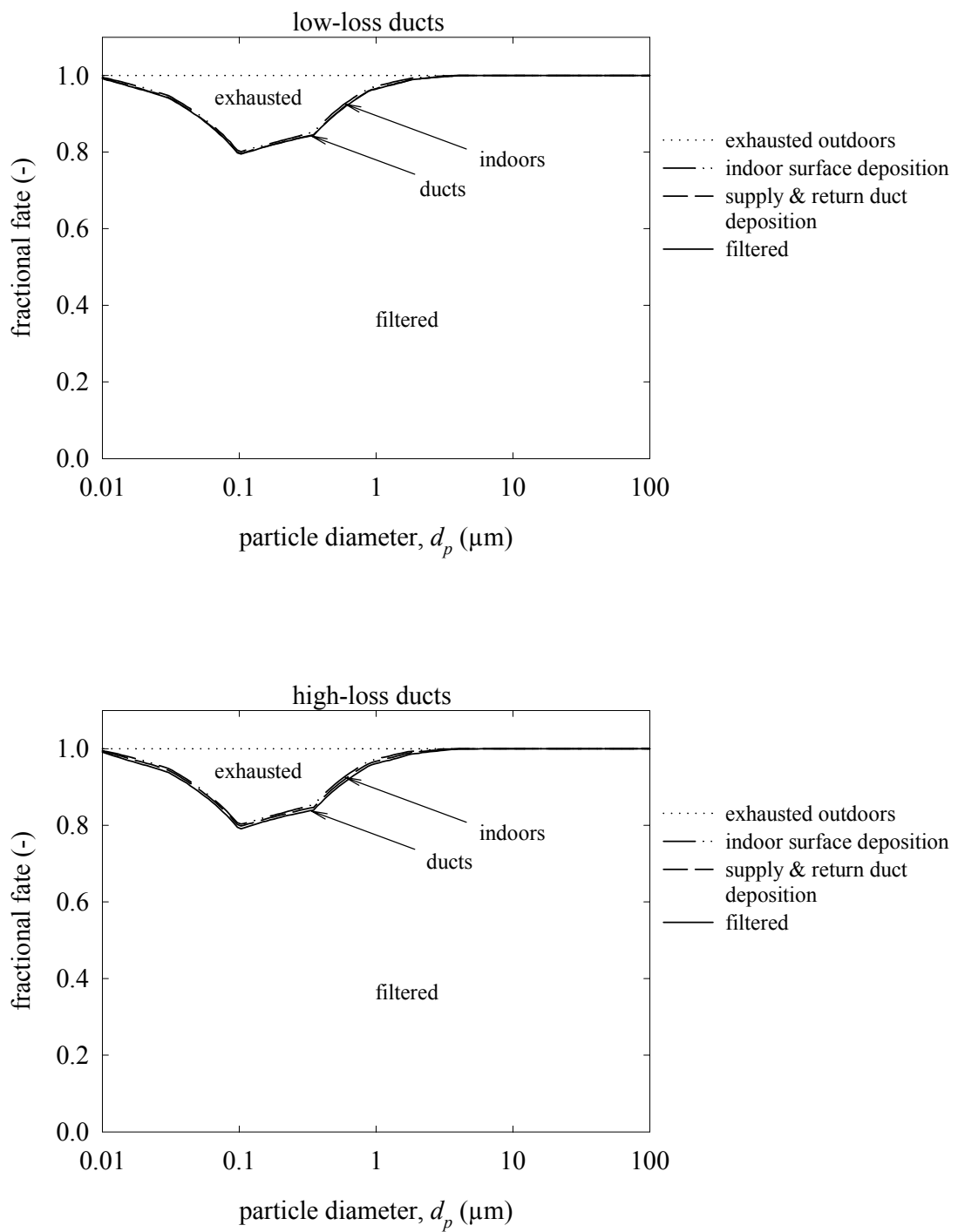
Figure 6.12 Predicted fractional fates of outdoor particles drawn into an air intake with ASHRAE 85% efficient filters for low-loss and high-loss ducts.
