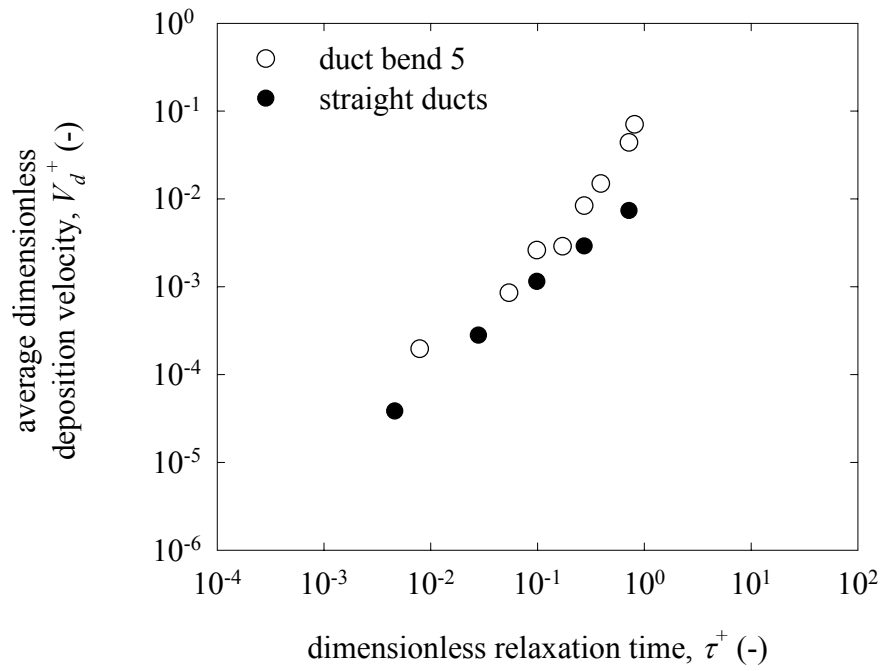
Figure 4.9 Composite dimensionless deposition velocities in bend 5 and in test ducts 1 and 2 versus dimensionless relaxation time at an air speed of 2.2 m/s.
