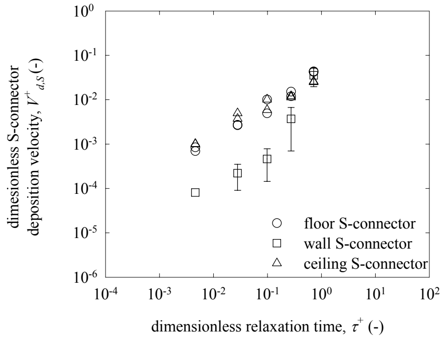
Figure 4.1 Dimensionless deposition velocities to S-connectors on the ceiling, wall and floor at an air speed of 2.2 m/s.
