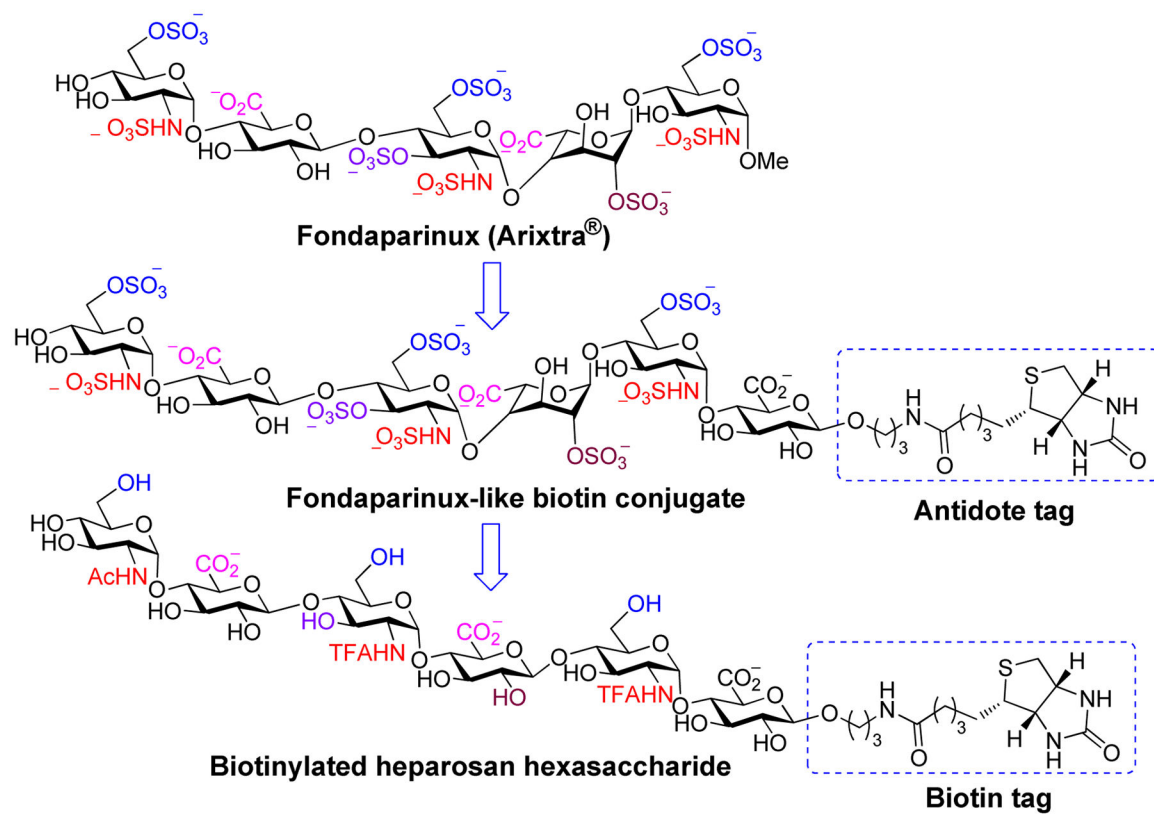
Figure 1. Fondaparinux (Arixtra®) and its analogues
