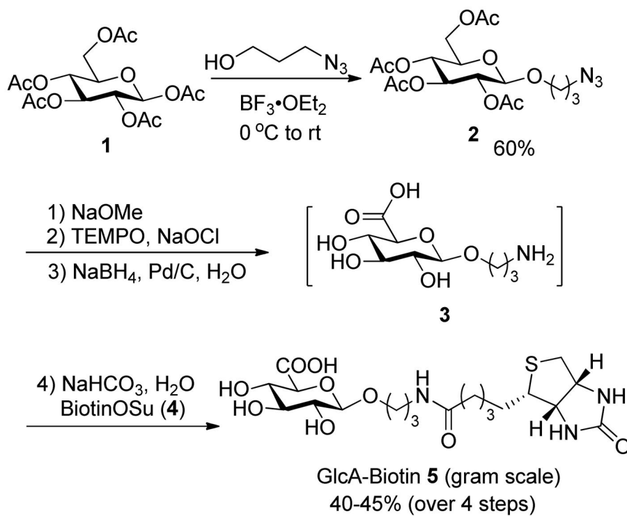
Scheme 1. Synthesis of GlcA-biotin conjugate 5
