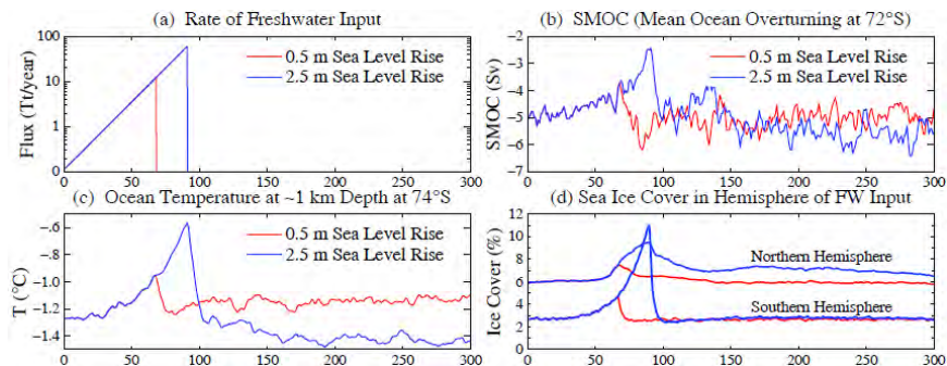
Fig. 13. (a) Freshwater input (Tt/year) to Southern Ocean (1 Tt = 1000 km 3 ). (b, c, d) Simulated overturning strength (Sv) of AABW cell at 72°S, temperature (°C) at depth 1.13 km at 74S, and sea ice cover (%).
