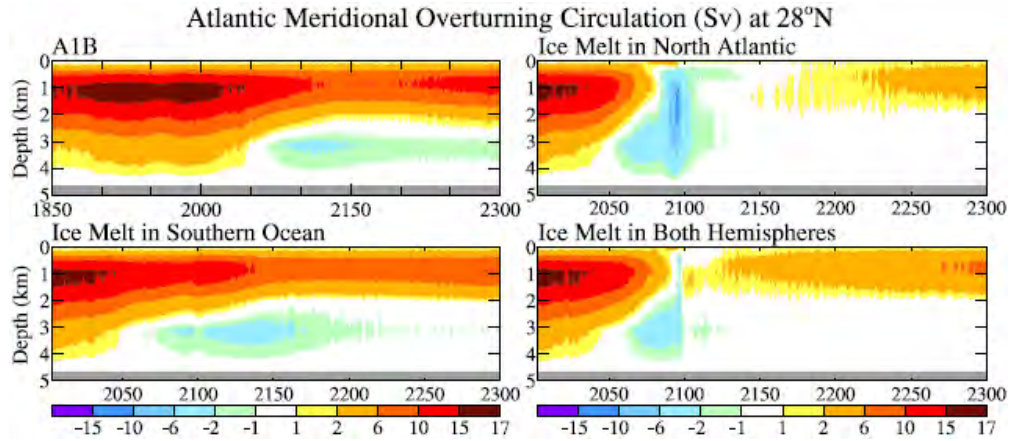
Fig. 9. Ensemble-mean AMOC (Sv) at 28N versus time for the same four scenarios as in Fig. 6, with ice melt reaching 5 m at the end of the 21 st century in the three experiments with ice melt.
