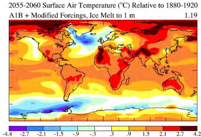
Fig. 16. Surface air temperature (°C) change relative to 1880-1920 in 2055-2060 for modified forcings.
