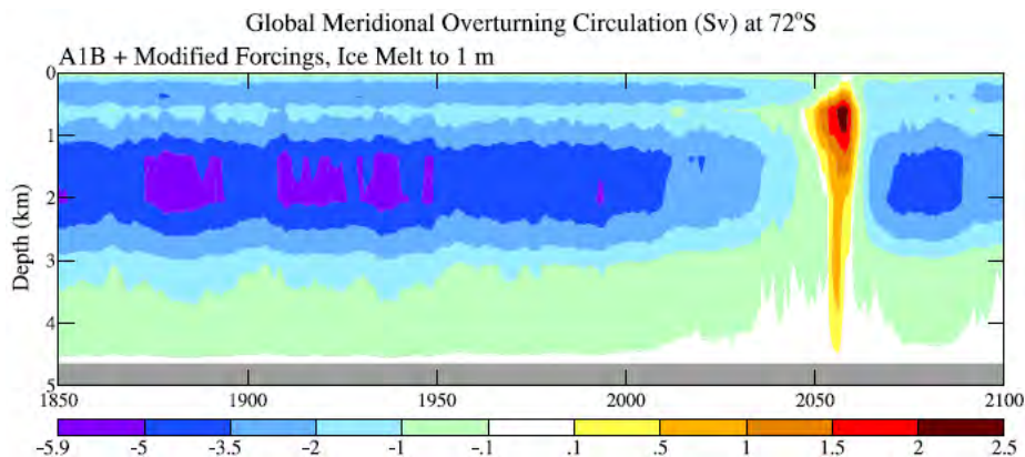
Fig. 17. SMOC, ocean overturning strength (Sv), including only the mean (Eulerian) transport. This is the average of a 5-member model ensemble for the modified forcing including advanced ice melt (720 Gt/year from Antarctica in 2011) and 10-year doubling.
