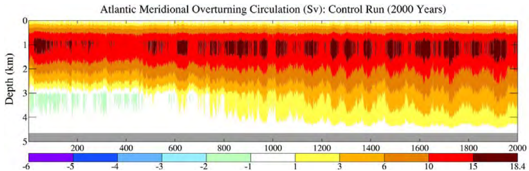
Fig. 3. Annual mean AMOC (Sv) at 28^\circ\text{N} in the model control run.
