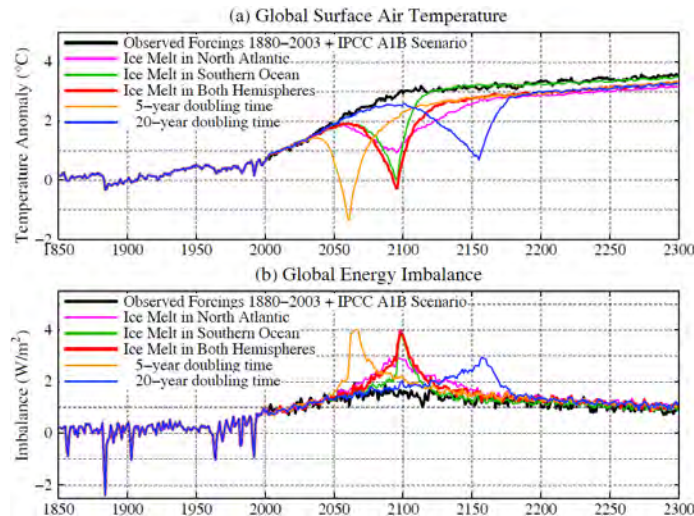
Fig. 7. (a) Surface air temperature ( ^{\circ}\text{C} ) relative to 1880-1920 for several scenarios. (b) Global energy imbalance ( \text{W}/\text{m}^2 ) for the same scenarios.
