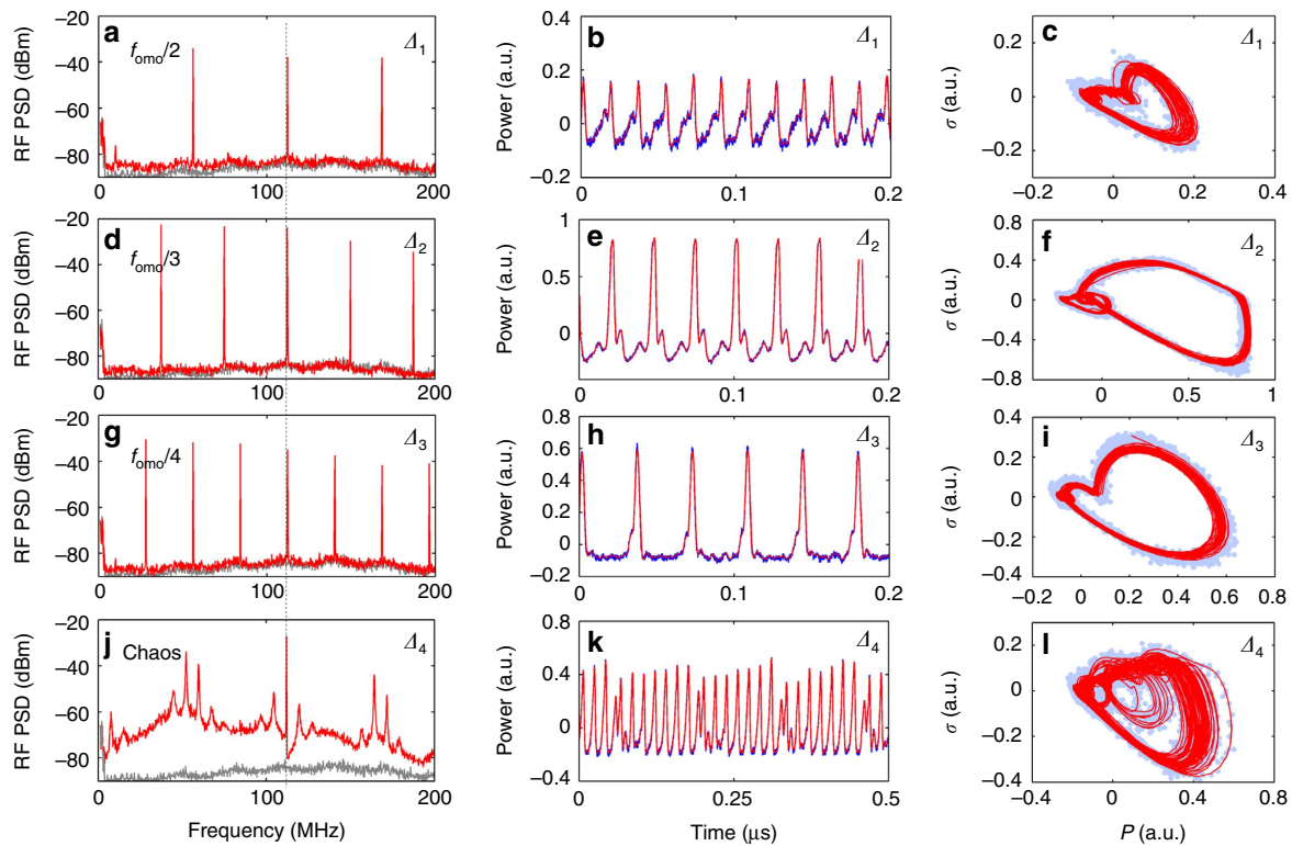
Figure 3 | Dynamical states under controlled drive conditions. (a–c) the f_{om0}/2 state ( \Delta_1 \approx 2.406 nm), (d–f) the f_{om0}/3 state ( \Delta_2 \approx 1.831 nm), (g–i) the f_{om0}/4 state ( \Delta_3 \approx 1.394 nm) and (j–l) the chaos state ( \Delta_4 \approx 2.285 nm) respectively. The curves (a,d,g,j) are the measured RF power spectral density (PSD) where the grey curves are the background noise floor. Notice the subharmonics have the background at the noise floor. The curves (b,c,e,f,h,i,k,l) are the temporal waveforms and orbital phase portraits, where the blue dots are the measured raw data and the solid red curves are the noise-reduced orbital trajectories.
