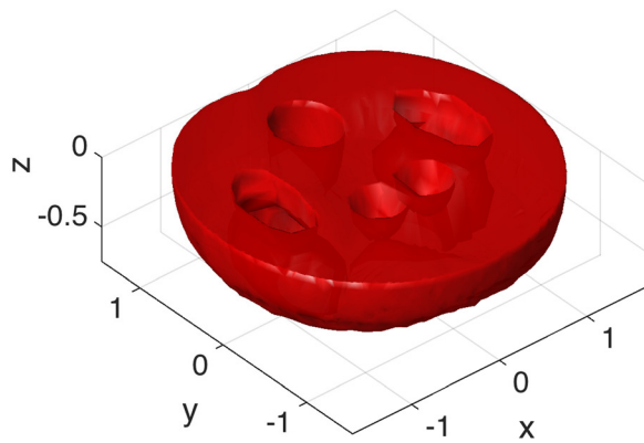
FIG. 7. A 3D visualization of the chaotic mixing region of a flow, demonstrating that the islands in the Poincaré maps extend as surfaces in three dimensions. This figure was produced by using a set of Poincaré sections to approximate the three-dimensional chaotic region, then using the MATLAB function alphavol 17 to produce the surface containing this region.
