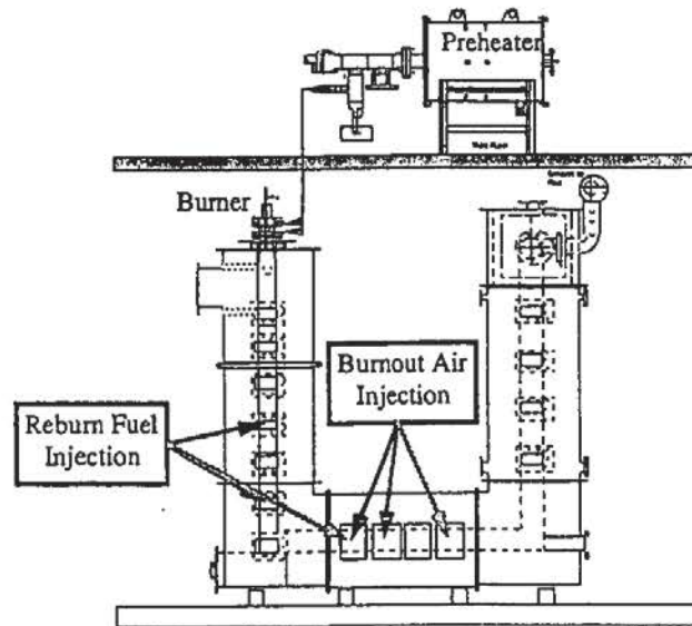
Figure 2. Pilot Scale Pulverized-Coal Fired Facility.
