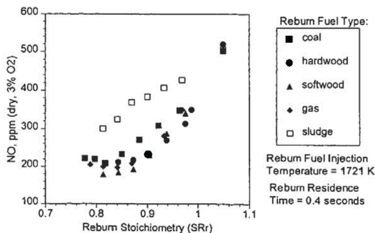
Figure 7. Reburn fuel comparisons at a reburn fuel injection temperature of 1721 K.
