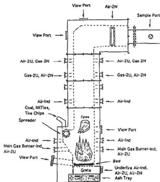
Figure 1. Pilot Scale Spreader-Stoker Facility.
