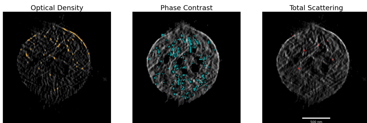
Figure 2. Tomography slices from 3D tomographic reconstructions of an \text{Al}_2\text{O}_3 catalyst particle with highlighted areas illustrating the segmentation process for identifying Ni nanoparticles. (left) Slice from the optical density reconstruction with high-density areas highlighted in orange. (middle) Slice from the phase contrast reconstruction with local minima highlighted in cyan. (right) Slice from the total scattering (i.e. optical density + phase) reconstruction that highlights the intersection of the previous two highlighted regions in red.
