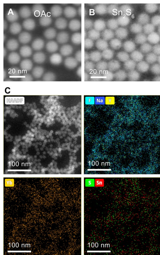
Figure 2. Nanoscale characterization of 14-nm \text{NaYF}_4 : 30% \text{Yb}^{3+} , 0.5% \text{Tm}^{3+} UCNP capped with \text{Sn}_2\text{S}_6^{4-} ligands. (A–B) Scanning transmission electron microscope images (STEM) of UCNP capped with (A) oleate ligands or (B) \text{Sn}_2\text{S}_6^{4-} ligands via direct ligand exchange. The center-to-center distances are 18.3 \pm 0.9 nm (oleate-capped) and 16.0 \pm 1.1 nm ( \text{Sn}_2\text{S}_6^{4-} -capped). (C) High-angle annular dark-field imaging (HAADF) STEM and EDS elemental maps of \text{Sn}_2\text{S}_6^{4-} -capped UCNP obtained via indirect ligand exchange.
