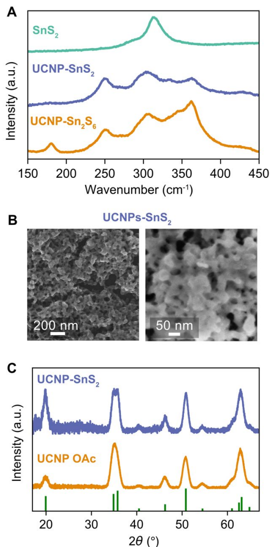
Figure 5. Annealing Sn 2 S 6 4- -capped 9-nm NaYF 4 : 8% Tm 3+ UCNPs at 350 °C to form a UCNP-SnS 2 nanocomposite. (A) Raman spectra of the Sn 2 S 6 4- -capped UCNPs before (orange line) and after (blue line) annealing. Also shown is the spectrum of the SnS 2 matrix formed by annealing Na 4 Sn 2 S 6 (green line). (B) SEM images of the UCNPs embedded in the SnS 2 matrix. (C) X-ray diffraction spectra of the UCNPs-SnS 2 nanocomposite (blue line) and oleate-capped UCNPs (orange line).
