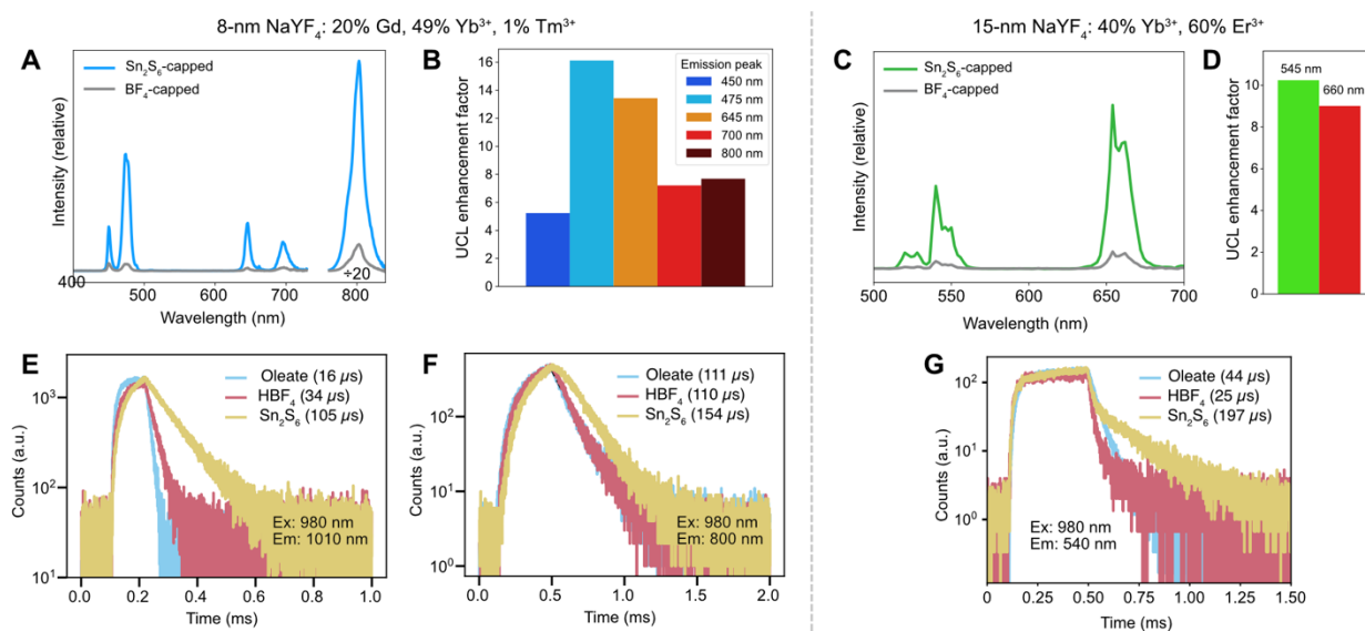
Figure 3. Upconversion luminescence (UCL) of Sn 2 S 6 4- -capped UCNPs. (A–D) UCL spectra and enhancement factors of Yb 3+ /Tm 3+ -doped (A–B) and Yb 3+ /Er 3+ -doped (C–D) UCNPs before and after adding Sn 2 S 6 ligands. (E–F) Fluorescence lifetimes of the 1010 nm (E) or 800 nm (F) emissions from 8-nm NaYF 4 : 20% Gd 3+ , 49% Yb 3+ , 1% Tm 3+ UCNPs with different surface treatments using 980 nm excitation. (G) Fluorescence lifetimes of the 540 nm emission 6-nm NaYF 4 : 20% Gd 3+ , 20% Yb 3+ , 2% Er 3+ UCNPs with different surface treatments using 980 nm excitation.
