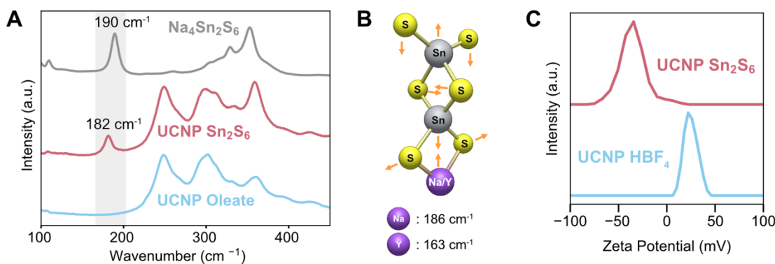
Figure 1. (A) Raman spectra of \text{Na}_4\text{Sn}_2\text{S}_6 and 14-nm \text{NaYF}_4 : 30% \text{Yb}^{3+} , 0.5% \text{Tm}^{3+} UCNPs capped with oleate or \text{Sn}_2\text{S}_6^{4-} ligands. (B) The relevant Raman-active vibrational mode of (\text{NaSn}_2\text{S}_6)^{3-} and (\text{YSn}_2\text{S}_6)^{3-} compounds and their vibrational energies. (C) Zeta potential of 15-nm \text{NaYF}_4 : 20% \text{Yb}^{3+} , 2% \text{Er}^{3+} UCNPs after ligand stripping and after \text{Sn}_2\text{S}_6 binding.
