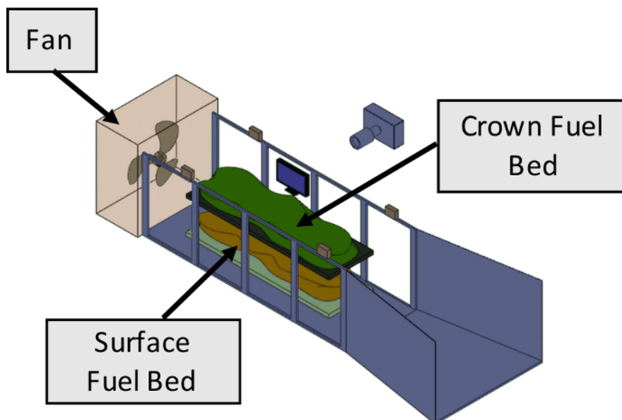
Figure 1: Wind tunnel experimental setup. Locations of the crown fuel bed, the surface fuel bed, and the tunnel fan have been labeled for convenience. The surface fuel bed is placed on the ground level of the wind tunnel over a standard scale. Representing the crown fuel bed, a fuel bed with chamise was placed over the surface fuel bed by suspending the fuel from a platform mounted on the wind tunnel frame. Please click here to view a larger version of this figure.
