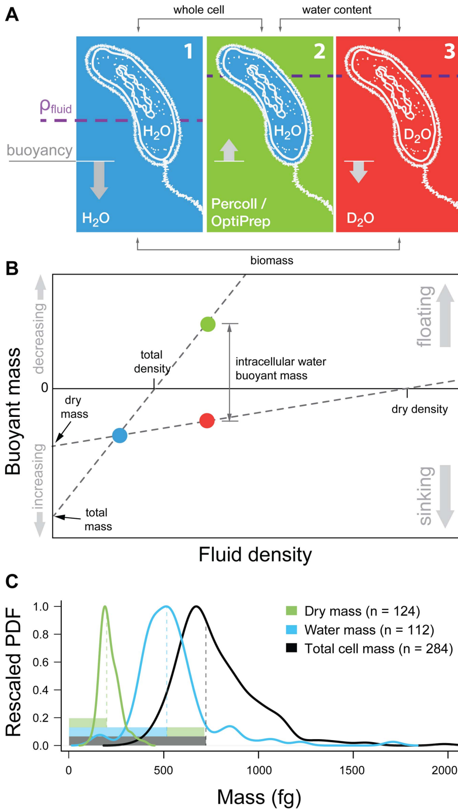
Figure 1. Buoyancy of a cell in fluids of different densities and membrane permeabilities. a ) In an H_2O or D_2O based fluid (1 or 3), the cell sinks as a result of the dry content's density being higher than the surrounding fluid. In a dense impermeable fluid (2), the buoyancy of the cell's water content dominates and the cell floats. b ) The pairing of the different buoyant mass measurements allows the determination of different biophysical parameters of the cell as shown in the plot (not to scale). c ) Kernel density estimates of probability densities for dry mass, water mass and total mass of a sample of fixed stationary-phase E. coli . Functions were rescaled so that their maxima were one. Solid bars represent sample medians. doi:10.1371/journal.pone.0067590.g001
