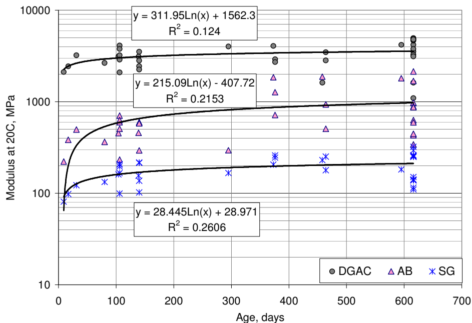
Figure 4.5: Temperature adjusted moduli of original sections versus age.
