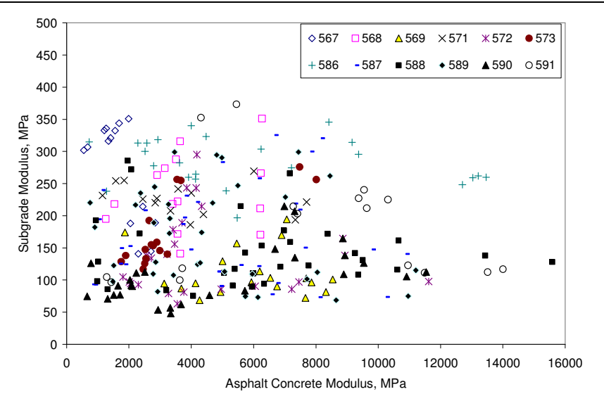
Figure 3.64: Variation of AC modulus with subgrade modulus.
