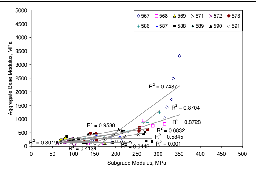
Figure 3.62: Variation of base and subgrade modulus in the trafficked area after HVS test.
