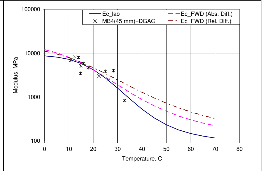
Figure 5.4: Composite AC moduli from laboratory and FWD tests for Section 589RF (MB4-G-45).
