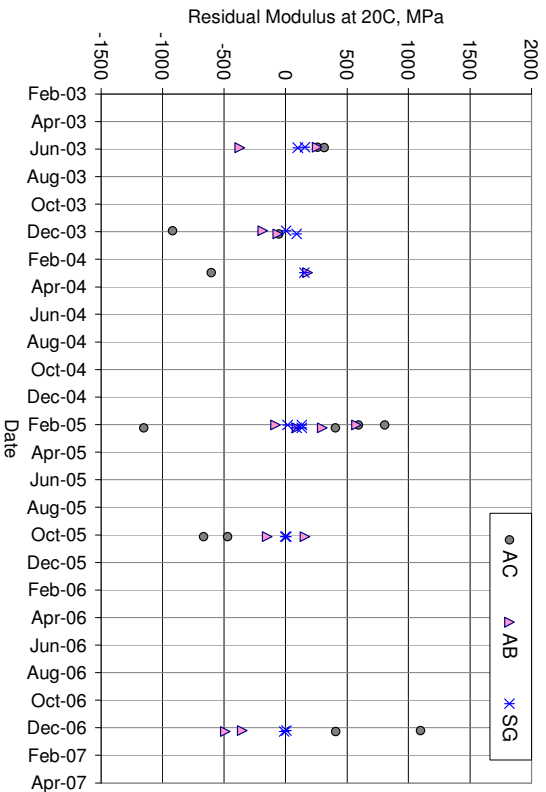
Figure 4.18: Time variation of residual moduli of Section 587RF (RAC-G).
