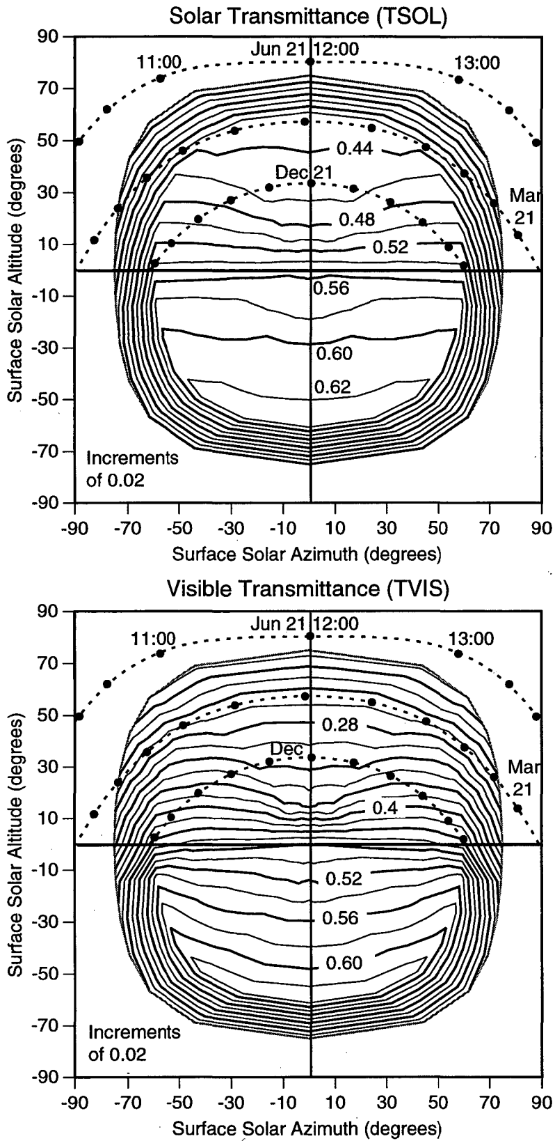
Figure 2. Single Pane Angular Selective Glazing TSOL and TVIS Distribution
