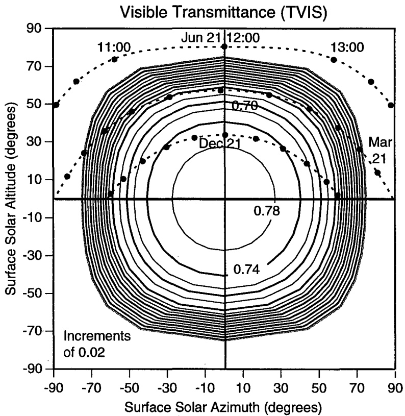
Figure 3. Single Pane Spectrally Selective Glazing TSOL and TVIS Distribution
