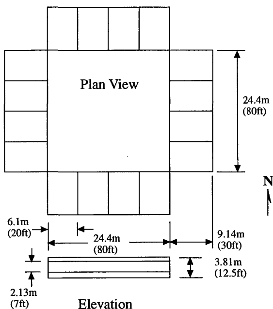
Figure 1. Commercial office building module used in the simulations. Each perimeter zone is partitioned into four offices, each 6.1 m x 9.1 m (20 ft x 30 ft). The core zone has a floor area of 594.6m 2 (6400ft 2 ).
