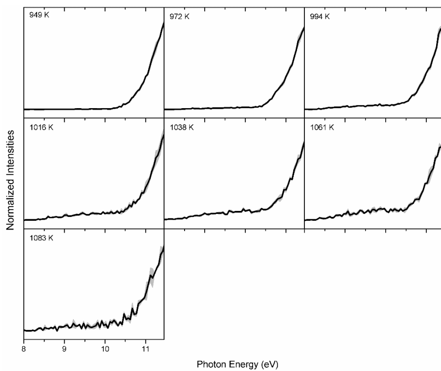
Figure S7. PIE measurement of m/z = 94 in the temperature from 949 K to 1083 K in NSRL. The PIE curves present sharp increase above 10.5 eV due to photolysis fragment of JP-10.
