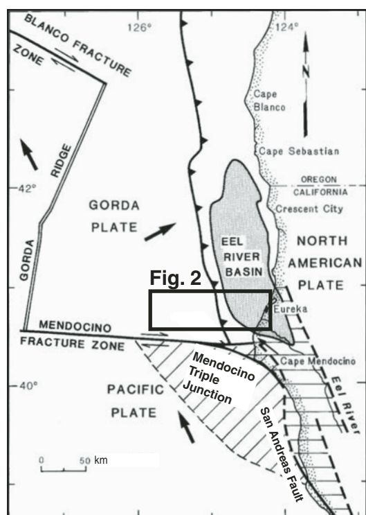
Figure 1. Regional map of offshore northern California showing major plate boundaries (after Clarke, 1992). The box roughly outlines the area shown in Figure 2.
